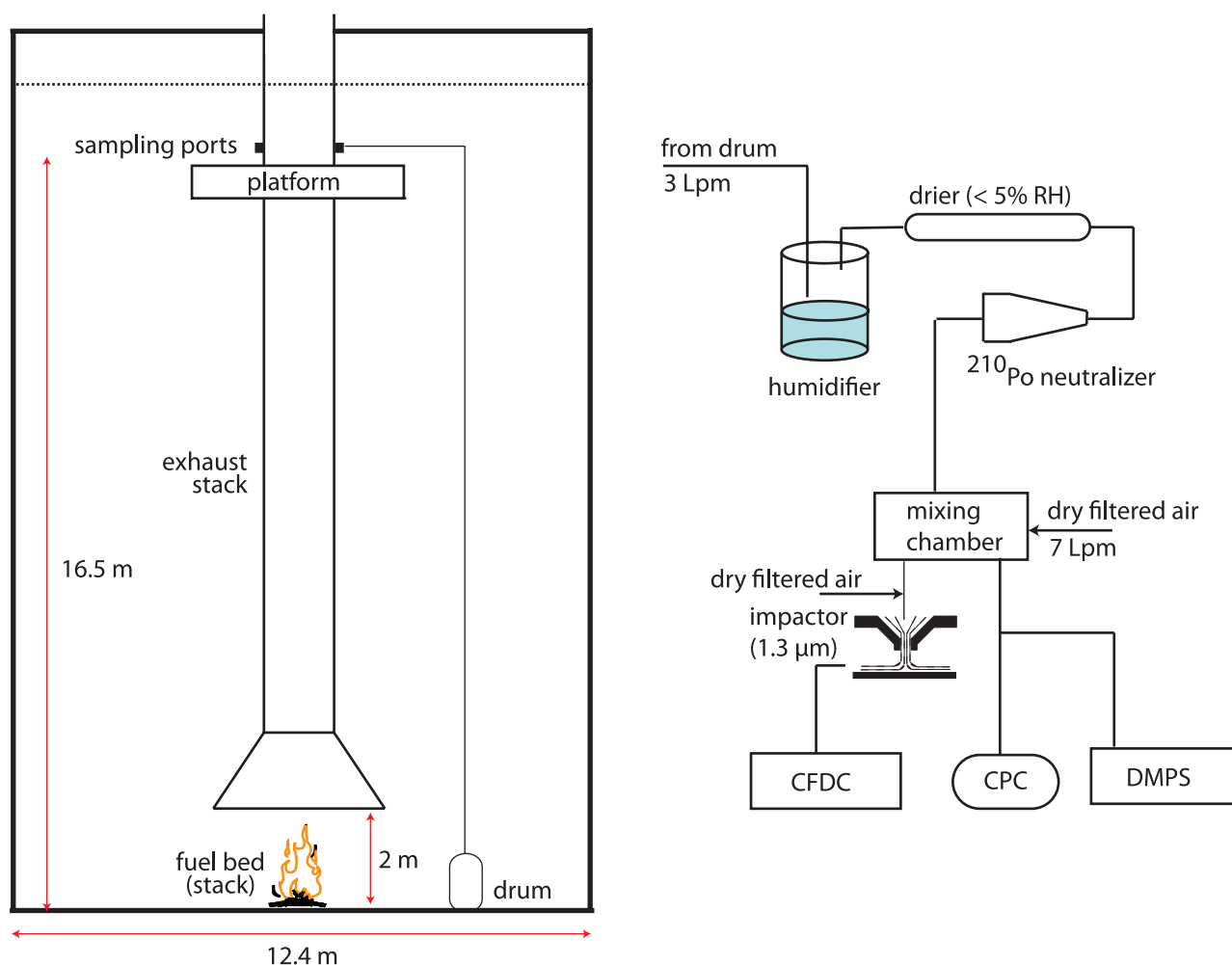
Figure 1. Schematic of the experimental setup. (left) Schematic of the Missoula Fire Sciences Laboratory. (right) Aerosol sampling strategy. Lpm, liters per minute.
