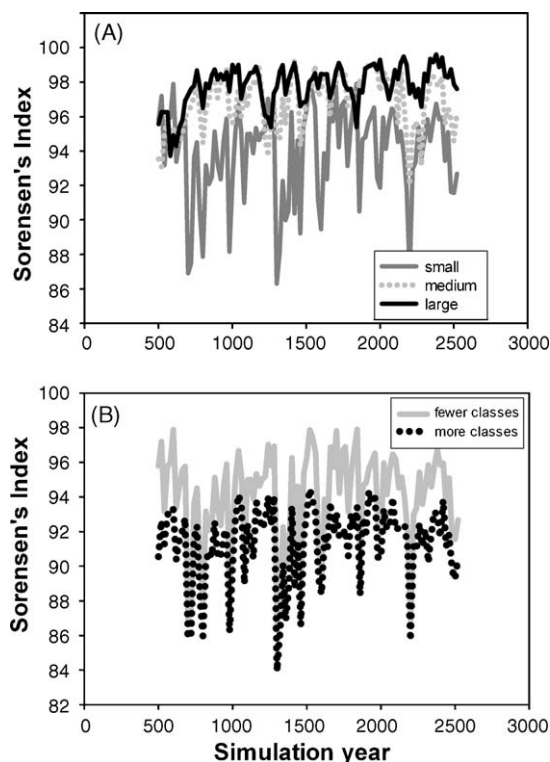
Fig. 5. The effect of the number of classes on calculation of Sorensen's Index where fewer classes denotes a simulation where only 20 classes (i.e., potential vegetation and succession class combinations) were used, and more classes represents a simulation using about 50 classes (Keane et al., 2008).
