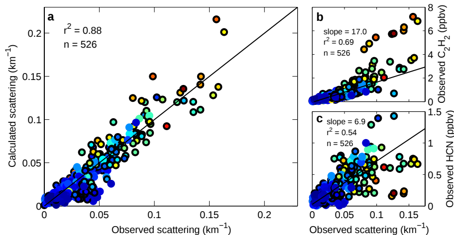
Fig. 8. Scatter plot for observed vs. reconstructed submicron scattering (a) . Associated scatter plots for submicron scattering vs. each tracer, [\text{C}_2\text{H}_2]^* (b) and [\text{HCN}]^* (c) . Lines are best fit to all data using total least squares (TLS) regression. Points are colored by [\text{toluene}]/[\text{C}_2\text{H}_2]^* , where red=1 and blue=0. Points with black border lie within the 3 \times 3 degree study area.
