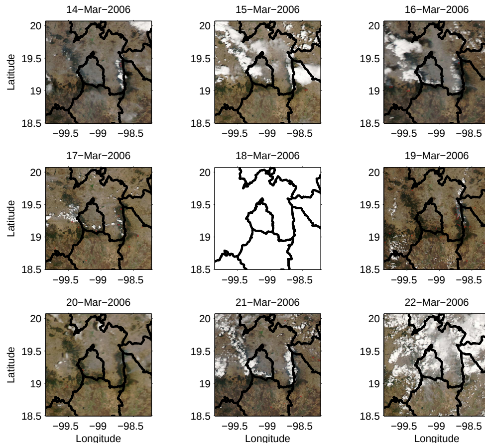
Fig. 11. MODIS-Aqua images around Mexico City for 14 March through 22 March 2006. Red boxes represent detected fires. Black lines are state boundaries. Blank areas represent missing data. Images courtesy of MODIS Rapid Response Project at NASA/GSFC.
