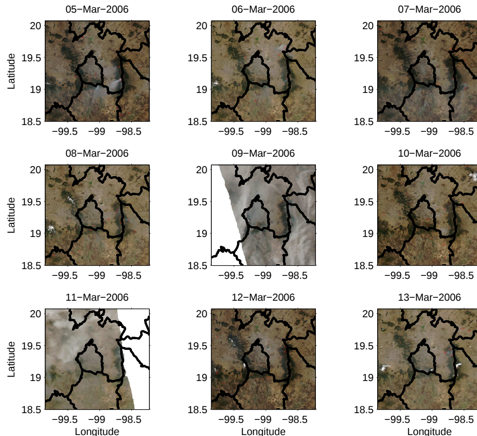
Fig. 10. MODIS-Aqua images around Mexico City for 5 March through 13 March 2006. Red boxes represent detected fires. Black lines are state boundaries. Blank areas represent missing data. Images courtesy of MODIS Rapid Response Project at NASA/GSFC.
