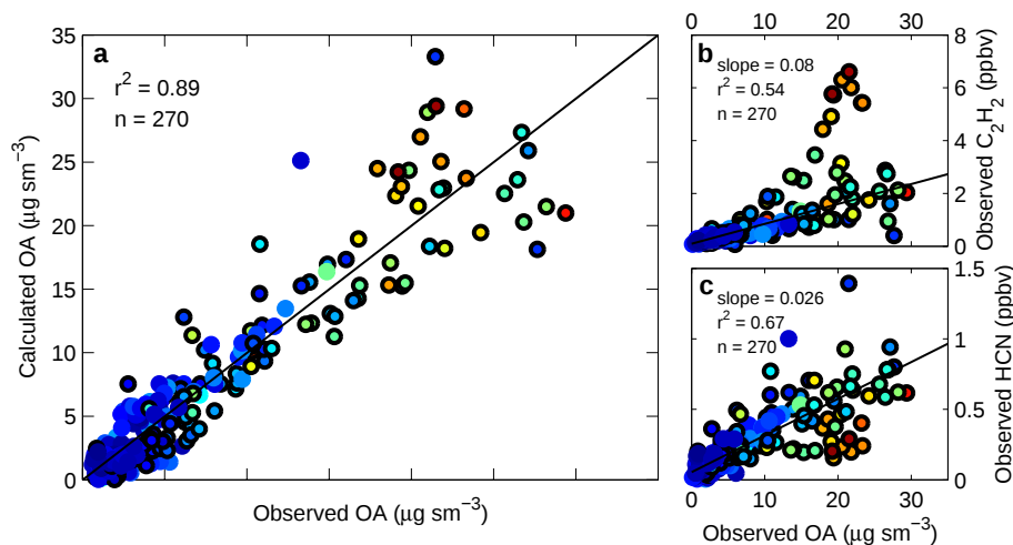
Fig. 5. Scatter plot for observed vs. reconstructed OA (a). Associated scatter plots for OA vs. each tracer, [\text{C}_2\text{H}_2]^* (b) and [\text{HCN}]^* (c). Lines are best fit to all data using total least squares (TLS) regression. Points are colored by [\text{toluene}]/[\text{C}_2\text{H}_2]^* , where red=1 and blue=0. Points with black border lie within the 3\times 3 degree study area.
