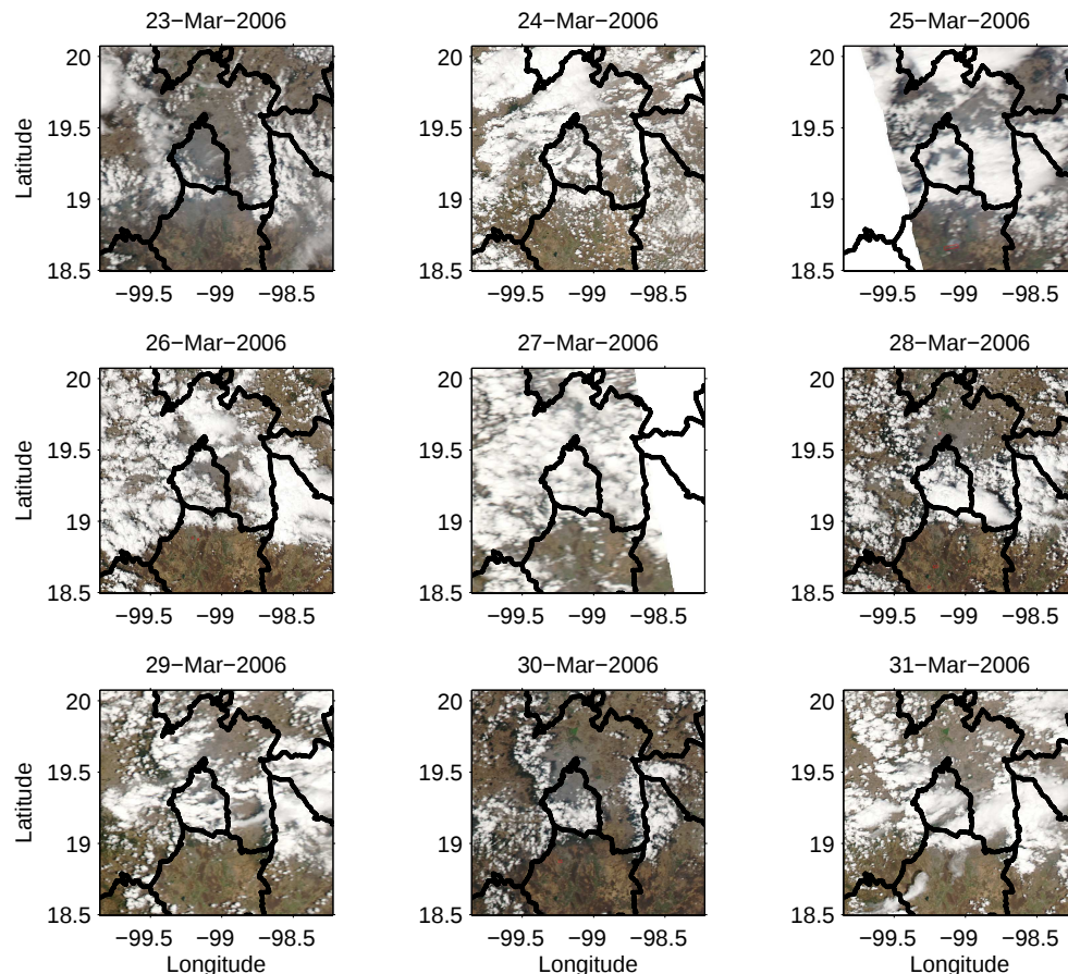
Fig. 12. MODIS-Aqua images around Mexico City for 23 March through 31 March 2006. Red boxes represent detected fires. Black lines are state boundaries. Blank areas represent missing data. Images courtesy of MODIS Rapid Response Project at NASA/GSFC.
