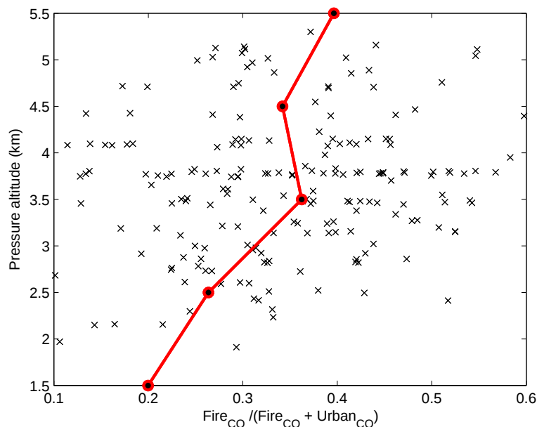
Fig. 9. Altitude dependence of fire CO over Mexico City. The fraction of excess CO (CO-background) which according to the two component analysis comes from biomass burning vs. pressure altitude for observations (black x symbols) made within the 3×3 degree study area around Mexico City. Note the ground level in MC is at 2.2 km pressure altitude. The mean values of data for 1 km bins are shown as black circles connected by the red line.
