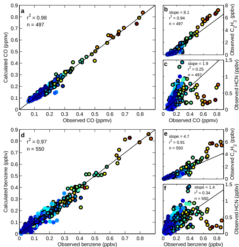
Fig. 4. Scatter plots for observed vs. reconstructed CO ( a ) and benzene ( d ). Associated scatter plots for CO vs. each tracer, [C_2H_2]^* ( b ) and [HCN]^* ( c ) and for benzene vs. each tracer, [C_2H_2]^* ( e ) and [HCN]^* ( f ). Lines are best fit to all data using total least squares (TLS) regression. Points are colored by [toluene]/[C_2H_2]^* , where red=1 and blue=0. Points with black border lie within the 3 \times 3 degree study area.
