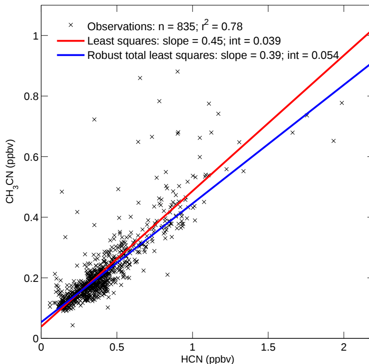
Fig. 6. Scatter plot of the HCN and the CH 3 CN observations made aboard the C-130 during the MILAGRO experiment ( r^2=0.78 ). The data (black x symbols) were fit using least squares (red: slope=0.45, intercept=0.039 ppbv), and robust total least squares (blue: slope=0.39, intercept=0.054) regression techniques.
