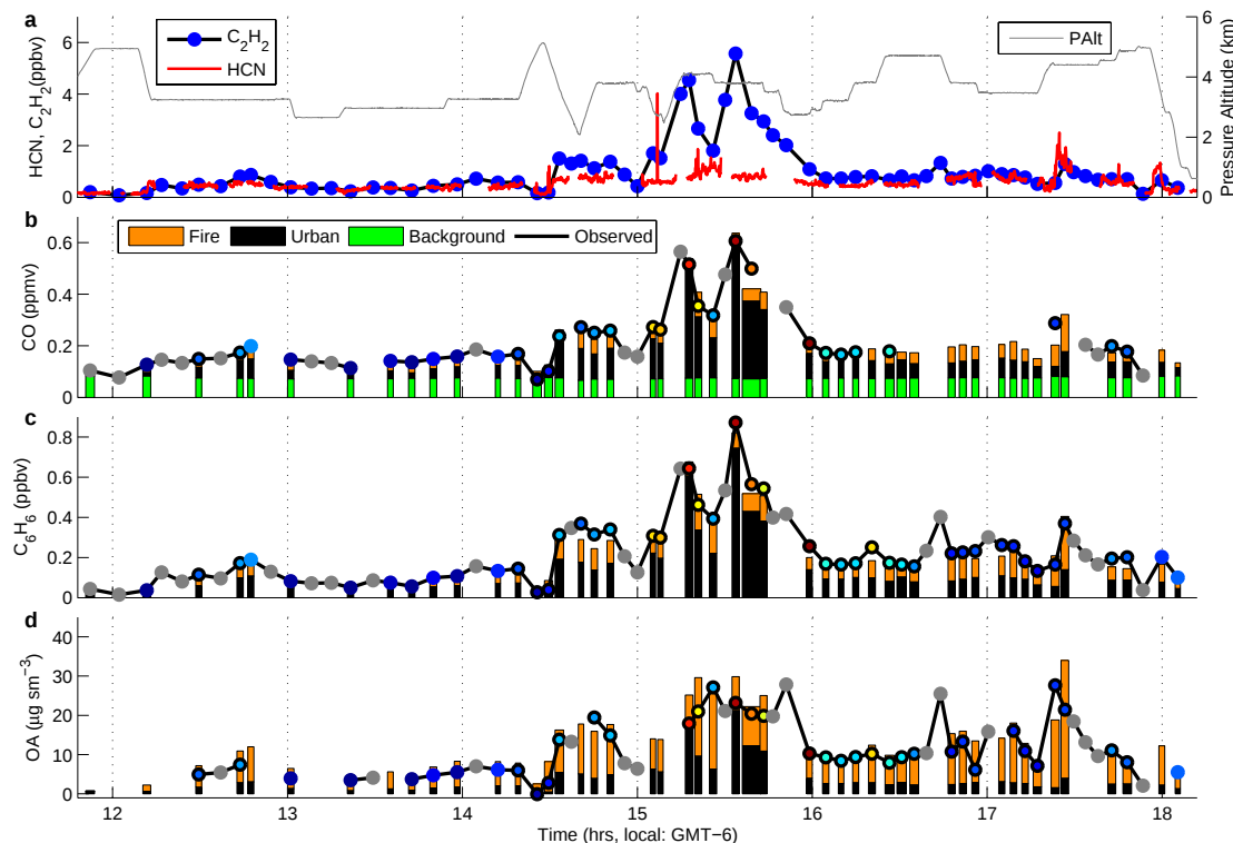
Fig. 3. Timeline from the flight of 8 March 2006: (a) measured HCN, C 2 H 2 , and pressure altitude. The observed (dots) and reconstructed (bars) CO, benzene, and organic aerosol concentrations, are shown in panels (b–d) , respectively. The bar widths represent the relative bottle sampling time (width has been expanded by 3× for clarity). The measurements in panels (b–d) are colored by [toluene]/[C 2 H 2 ]* with color scale ranging from red=1 to blue=0, and grey meaning data was unavailable for this calculation. Data points with black borders in panels (b–d) lie within the 3×3 degree study area.
