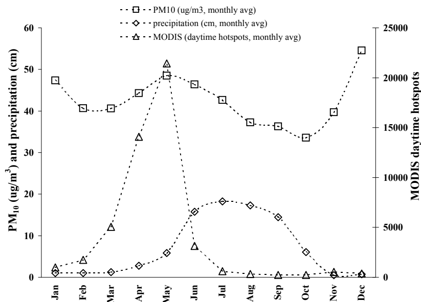
Fig. 6. Time series of monthly average PM 10 (Pedregal RAMA station 2003–2008 average, www.sma.df.gob.mx/simat/cambia_base.htm ); MODIS daytime hotspots for Mexico (2003–2008 average, www.conabio.gob.mx ); and monthly average precipitation for MCMA (see Sect. 4.2).
