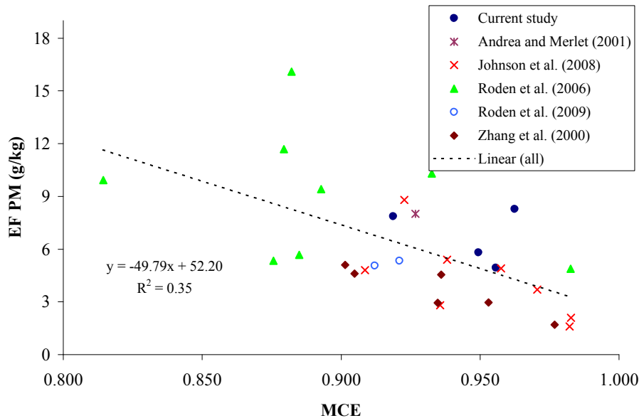
Fig. 3. Variation of the particle emission factor with MCE for open wood cooking fires.
