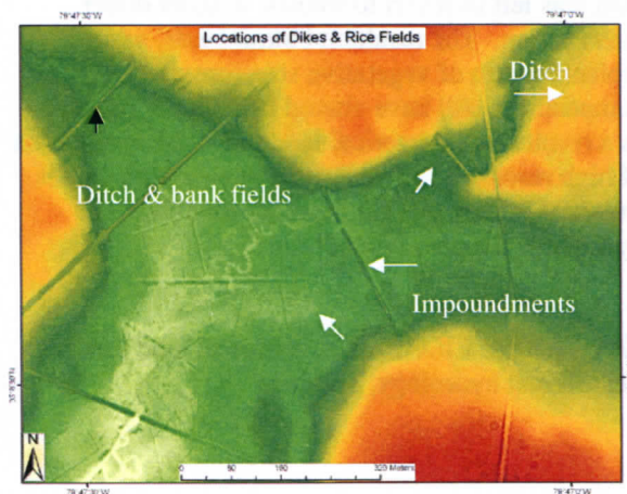
Figure 2. Depiction of surface topography derived from Lidar data for a section of Huger Creek, Santee Experimental Forest. The location of some impoundments, ditches and ditch and banked fields are noted.
