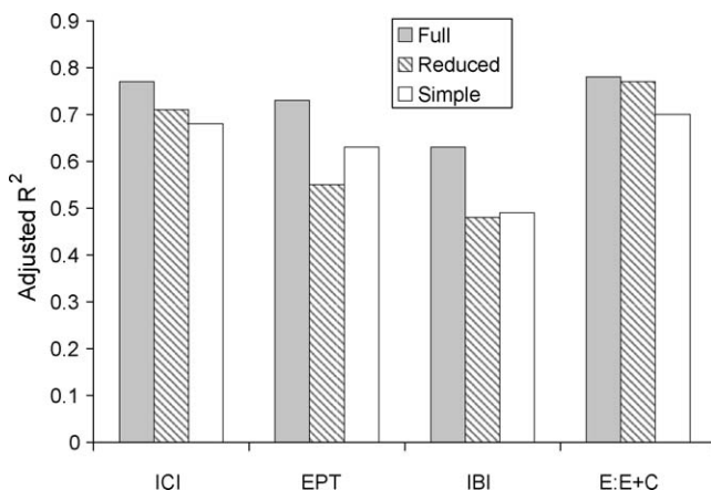
Fig. 3. Predictive power (adjusted R^2 ) of full, reduced, and simple models for selected macroinvertebrate and fish measures of biotic integrity.
