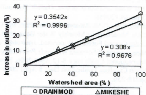
Fig.3 Effect of land use change on outflow.
