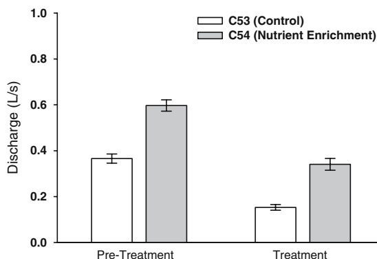
Figure 2. Mean daily stream discharge ( \pm 1 S.E.) for C53 (control) and C54 (treatment) for pre-treatment (May 1999–June 2000) and treatment (July 2000–March 2001) periods at the Coweeta Hydrologic Laboratory, Macon Co., North Carolina, USA.
