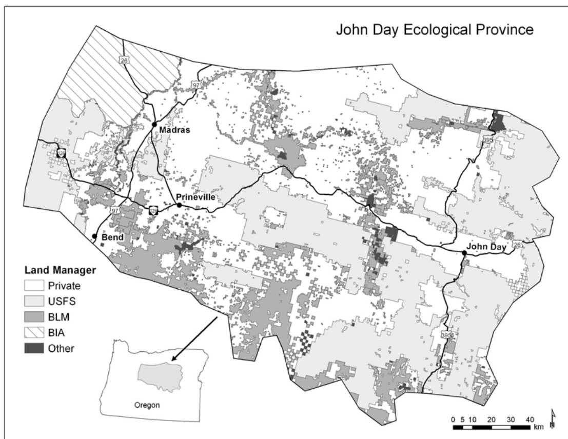
Figure 3 —Location of the John Day Ecological Province in central Oregon. Land managers are as follows: USFS = USDA Forest Service, BLM = USDI Bureau of Land Management, BIA = USDI Bureau of Indian Affairs, and Other, including Oregon Department of State Lands and USDI Fish and Wildlife Service.
