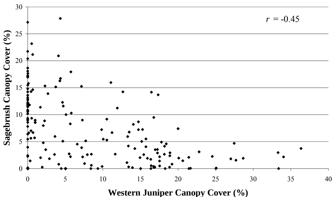
Figure 5 —Canopy cover of western juniper trees and sagebrush (all taxa combined) on plots within seven strata sampled in the John Day province, central Oregon, 2007 ( n = 178 ). (See table 1 for strata descriptions).
