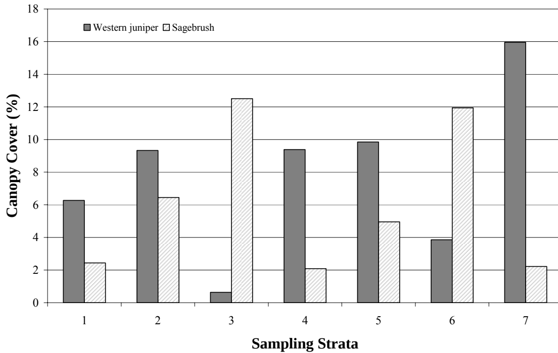
Figure 4 —Canopy cover (%) of western juniper trees and sagebrush in plots sampled in the John Day province, central Oregon, 2007 ( n = 178 ). Strata are defined as follows: 1 = non-sagebrush, far from juniper stands, 2 = other sagebrush, far from juniper stands, 3 = low/mountain big sagebrush, far from juniper stands, 4 = non-sagebrush, near juniper stands, 5 = other sagebrush, near juniper stands, 6 = low/mountain big sagebrush, near juniper stands, and 7 = juniper stands. Far from juniper stands = > 1,600 m; near juniper stands = \leq 1,600 m.
