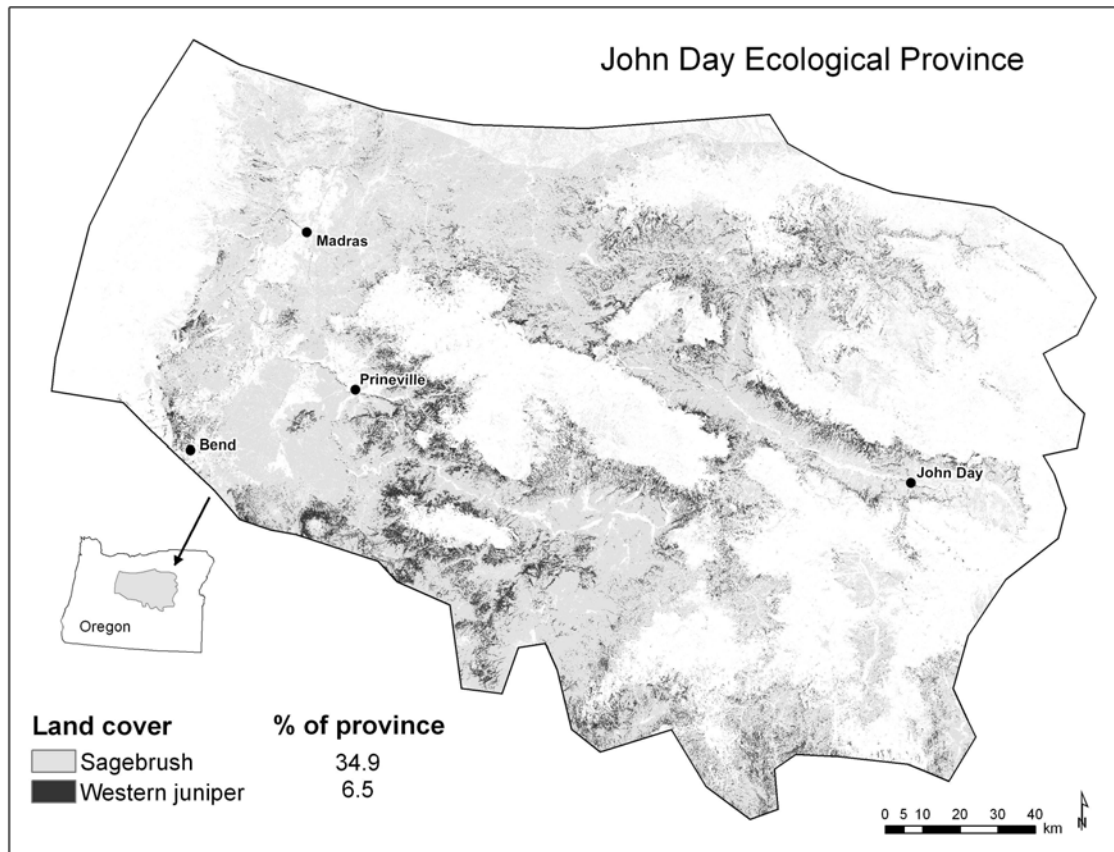
Figure 2 —Western juniper and sagebrush (all sagebrush ecological systems combined) as mapped by LANDFIRE in the John Day Ecological Province, central Oregon. See text for details.
