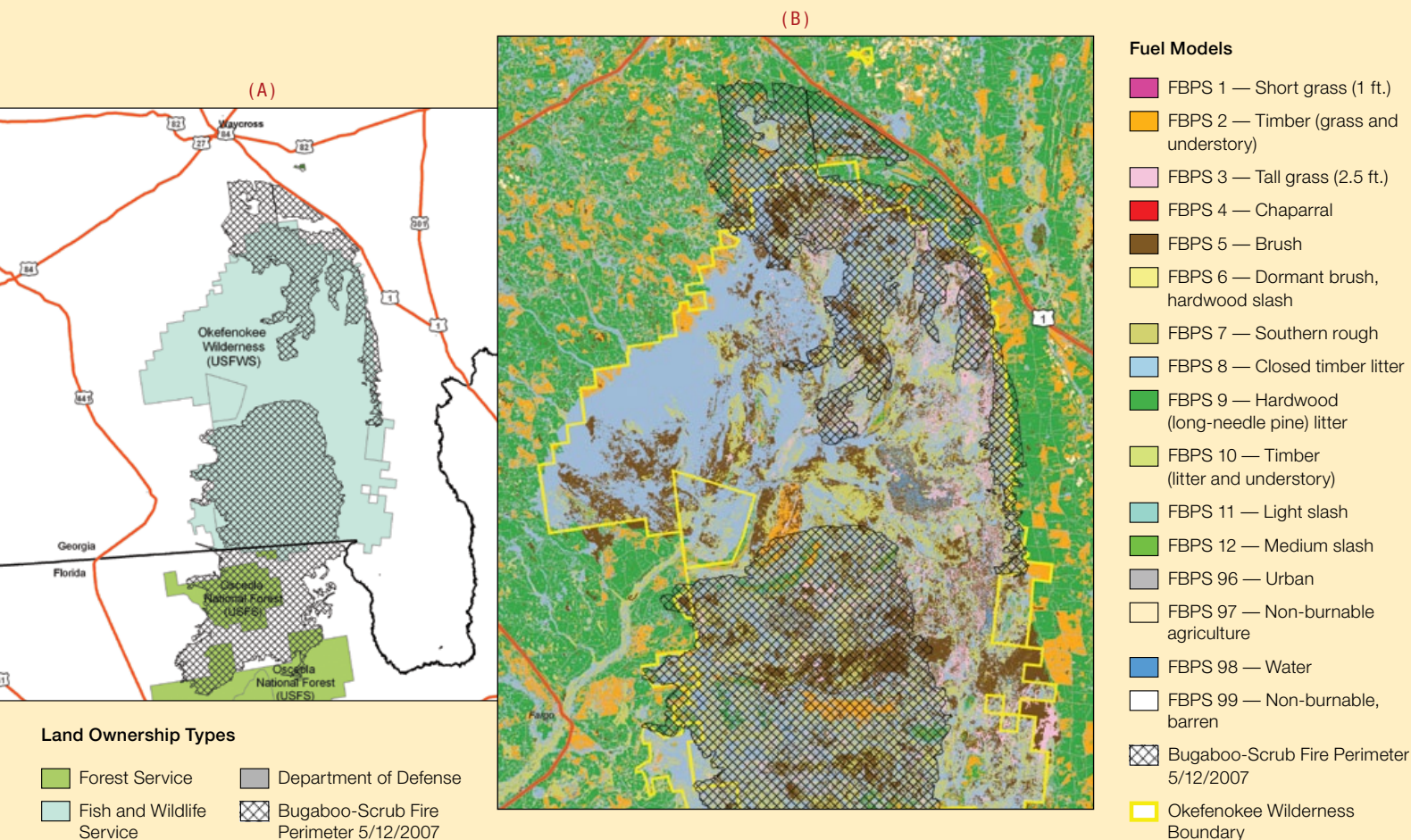
FIGURE 23. The perimeter of and land ownership types involved in the Georgia Bay Complex/Bugaboo Fire of 2007 (A) and the Southern Wildfire Risk Assessment surface fuel model map (B) that was used to plan firefighting efforts in the Okefenokee National Wildlife Refuge.
