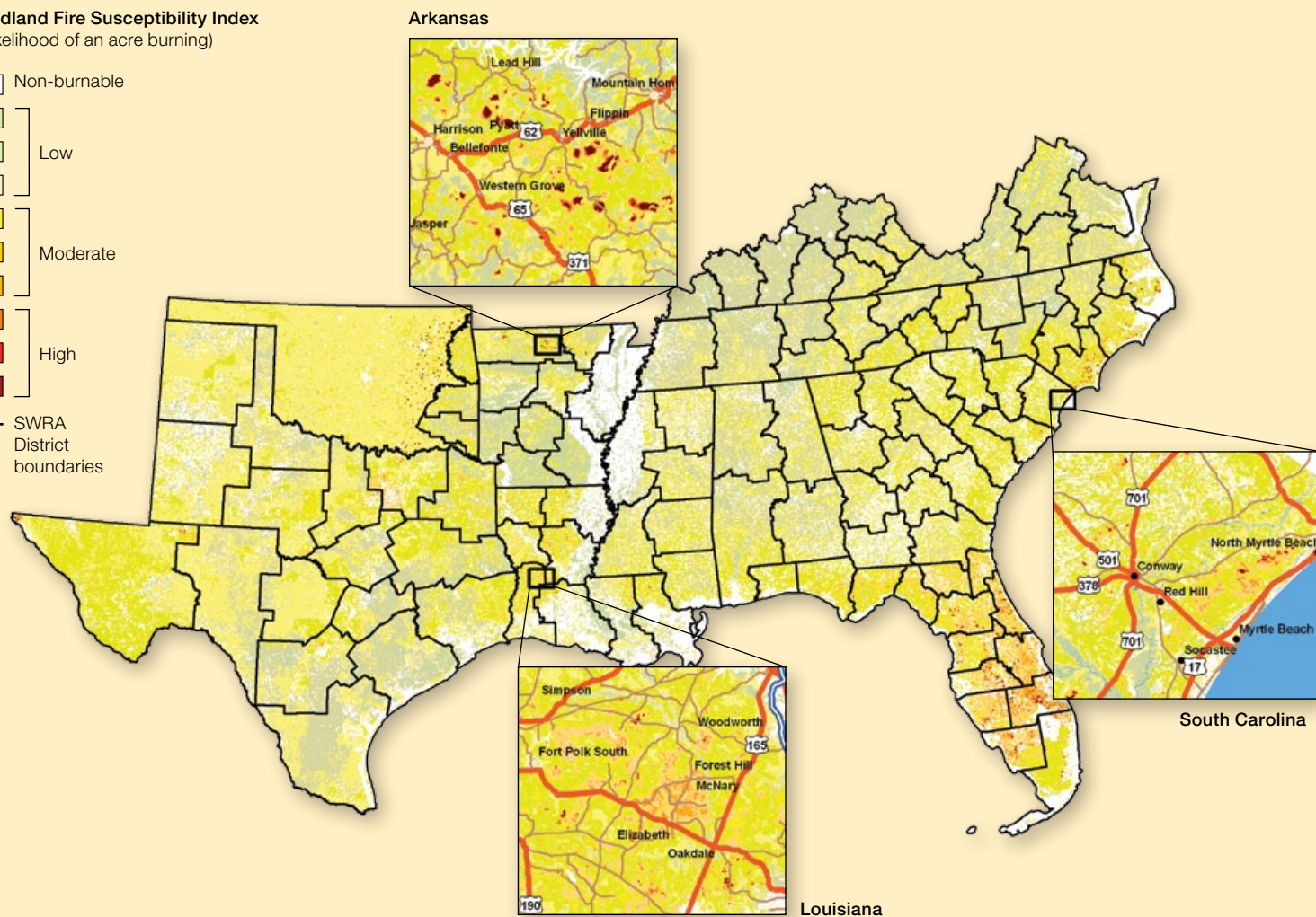
FIGURE 7. The regionwide potential for wildfire, based on the likelihood of each acre burning, with three local examples in Arkansas, Louisiana, and South Carolina. The local examples clearly show that many areas with moderate to very high probability of wildfire are close to communities and valuable infrastructure.
