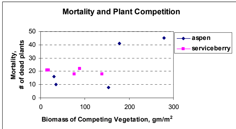
Figure 3. Relationship of plant mortality to biomass of competing vegetation. Plots with the highest aspen mortality were from the Yoast site.
