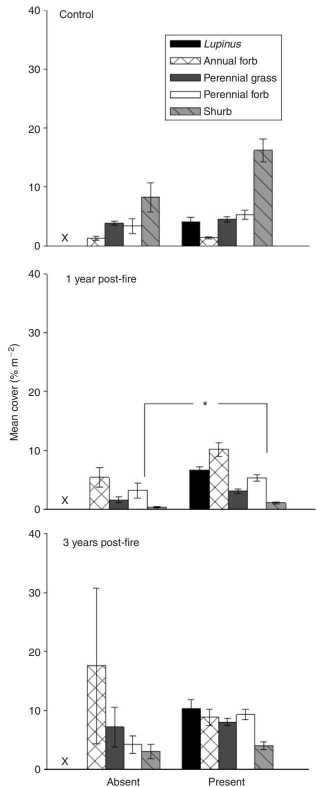
Fig. 5. Functional group response to time since fire in the absence and presence of Lupinus for the unburned control, 1-year post-fire and 3-years post-fire treatments. Values are mean cover \pm s.e. n = 28 –35 plots per treatment per block; asterisk indicates significant differences between Lupinus absence or presence within burn treatment at P < 0.05 .
