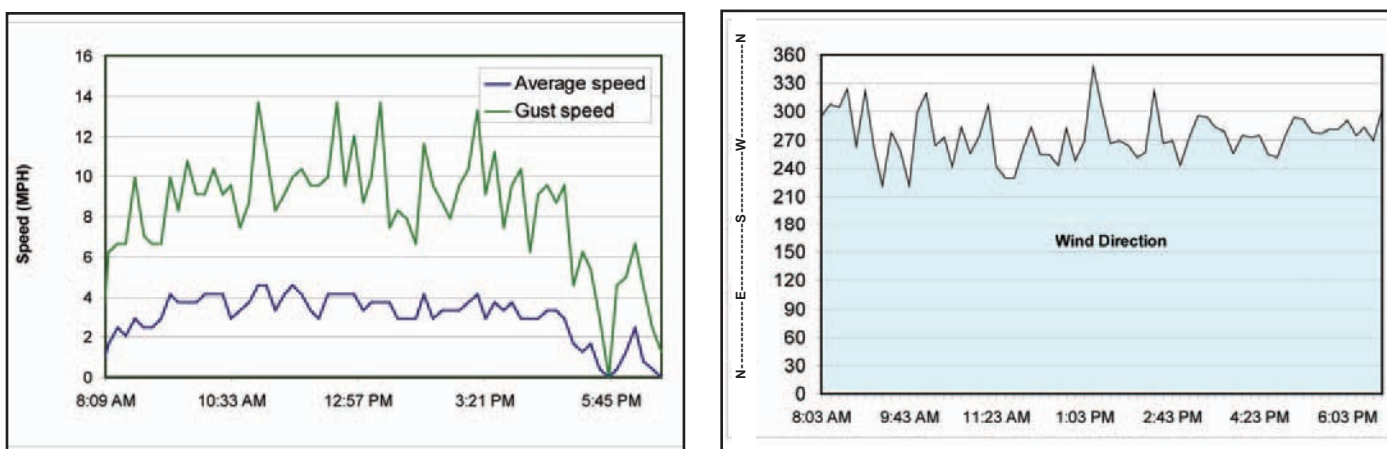
Figure 4—Wind speed (left) and wind direction (right) measured in the front field.
