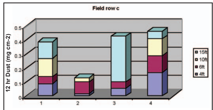
Figure 10 (left – woods) Figure 11 (right – field)—Accumulation of dust particles along a 200m transect and at 50m and 100m away from the source. Note the differences in y-axis scales.
