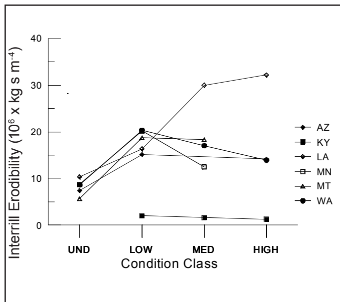
Figure 22—Interrill erodibility.
