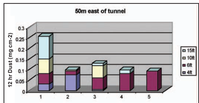
Figure 12—Dust movement off the trail into the forest along the tunnel trail. Note the differences in y-axis.
