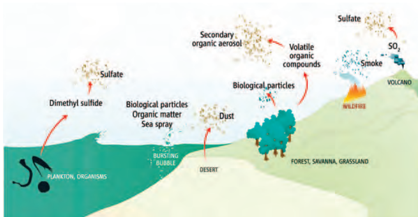
Figure 1.1. Sources of aerosol particles to the natural atmosphere: Primary particles—such as sea spray, soil dust, smoke from wildfires, and biological particles including pollen, microbes, and plant debris—are emitted directly into the atmosphere. Secondary particles are formed in the atmosphere from gaseous precursors; for example, sulfates are formed from biogenic dimethyl sulfide and volcanic sulfur dioxide ( \text{SO}_2 ), as well as, secondary organic aerosol from biogenic volatile organic compounds. (Reprinted with the permission of Andreae 2007 and the American Association for the Advancement of Science (AAAS). Copyright: AAAS, 2007.)
