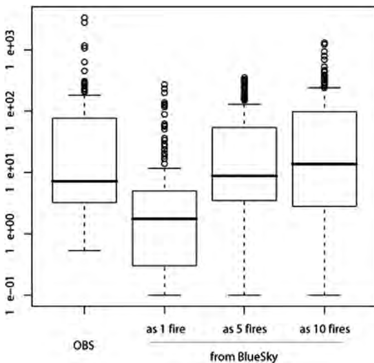
Figure 22.8. PM 2.5 concentrations near Twisp, Washington, for the Rex Creek fire for the period of August 19–26, 2001. Box-whisker plots show observed concentrations (OBS) and BlueSky concentrations for the one-fire, five-fire, and ten-fire cases. Values below 0.1 are set to 0.1 for plotting purposes.
