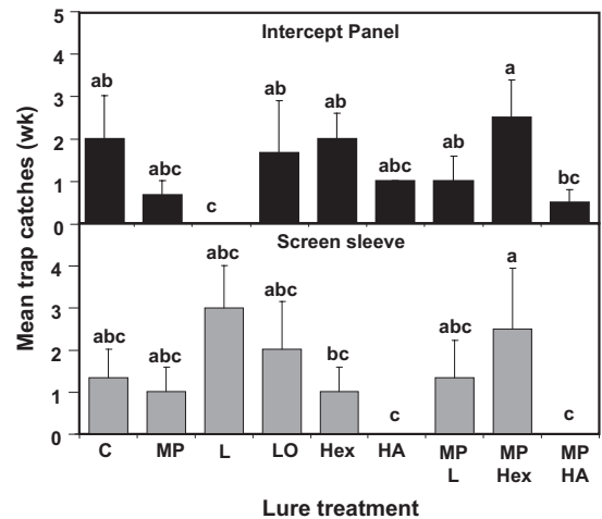
Fig. 7. Mean trap catches per week per lure for the Intercept panel (top) and screen sleeve (bottom) traps. Error bars represent SEM. Letters over bars represent significantly different means within lure treatments at the 95% confidence level. [C, control; MP, A. glabripennis male pheromone blend; L, (-)-linalool; LO, linalool oxide; Hex, (Z)-3-hexen-1-ol; HA, (Z)-3-hexenyl acetate; MPL, male pheromone blend + (-)-linalool; MPHex, male pheromone blend + (Z)-3-hexen-1-ol; MPHA, male pheromone blend + (Z)-3-hexenyl acetate; ref. Table 1 for amounts].
