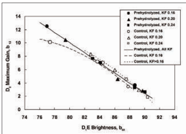
4. Maximum possible brightness gain in the D_2 stage vs. the brightness of the pulp entering the stage.
