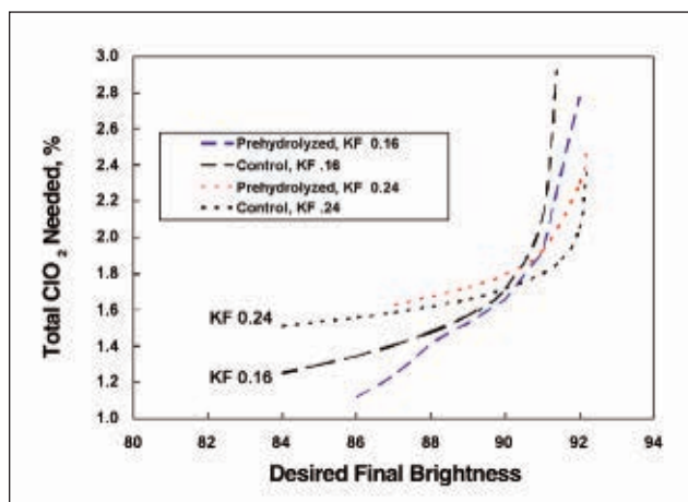
7. Minimum \text{ClO}_2 requirement vs. final brightness target. D(E)D sequence.
