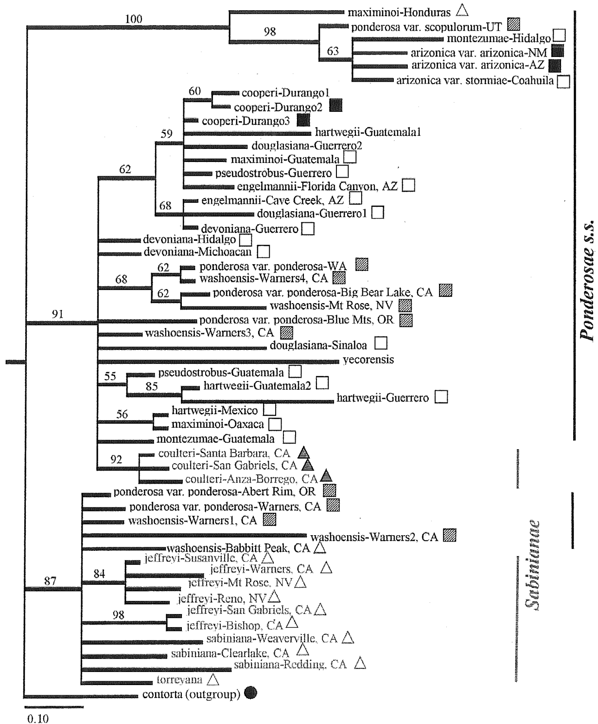
Fig. J. Bayesian majority-rule consensus tree for WD-40 showing only nodes with \geq 9 ; posterior probabilities or higher and supported by parsimony bootstrap greater than 50. Numbers are bootstrap proportions from parsimony analysis. Branches are proportional to length; scale bar is substitutions per site. See Fig. 6a for trnG haplotype symbols.
