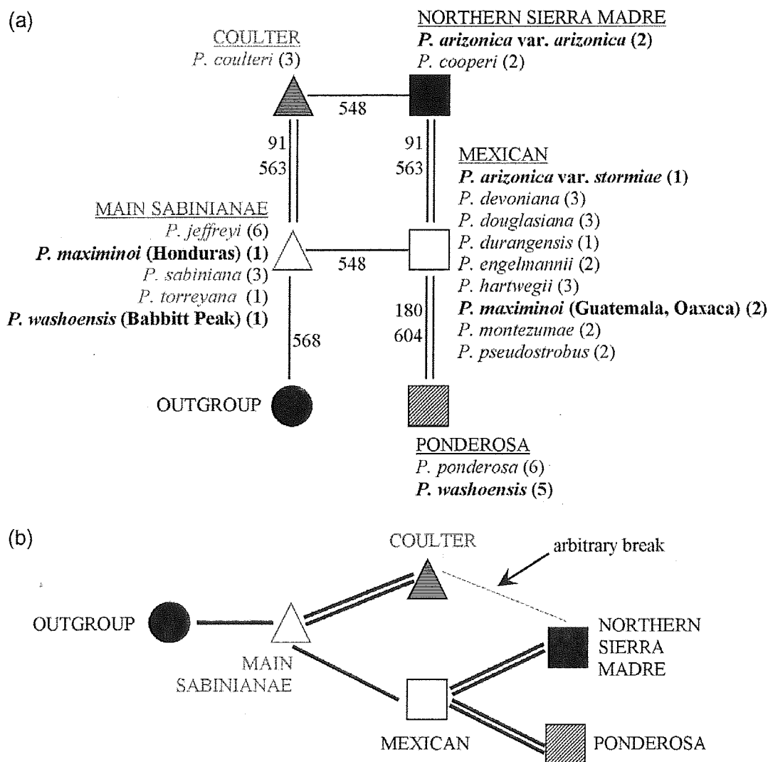
Fig. 6. (a) Chloroplast trnG haplotype network. Single and double lines represent one and two nucleotide substitutions, respectively, at six aligned positions: 91, 180, 548, 563, 568, and 604. Number of accessions in parenthesis. Species with more than one haplotype are in bold. (b) Arbitrarily resolved network (see Section 3.5).
