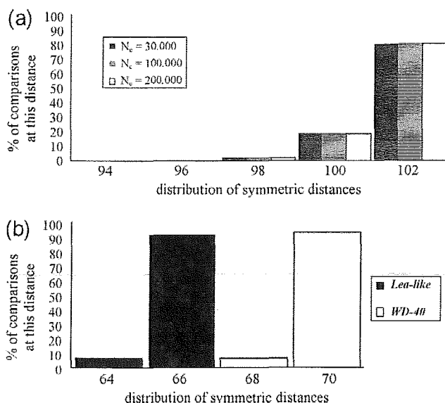
Fig. 7. Distribution of symmetric distances for gene trees simulated using a simple coalescent model within a species tree; (a) within 'clouds' of gene trees simulated for three levels of effective population size ( N_e ); (b) from the LEA-like consensus gene tree and from the WD-40 consensus gene tree to the cloud of trees simulated using N_e = 100,000 .
