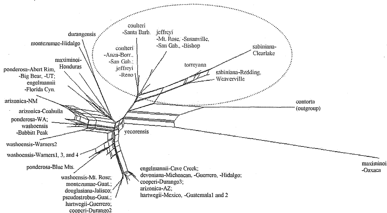
Fig. 4. LEA-like neighbor-net network created using maximum likelihood distances. Oval highlights clade that contains four Sabiniana species.
