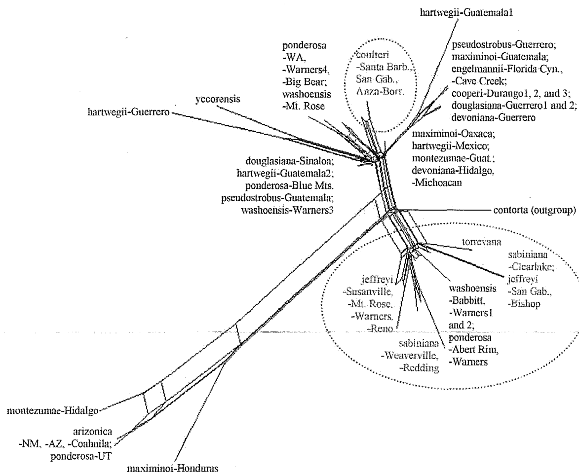
Fig. 5. WD-40 neighbor-net network created using maximum likelihood distances. Ovals highlight two clades that contain the four Sabiniana species.
