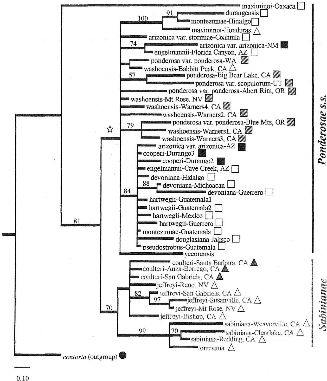
Fig. 2. Bayesian majority-rule consensus tree for LEA-like showing only nodes with 0.95 posterior probabilities or higher. Numbers are bootstrap proportions from parsimony analysis. Branches are proportional to length; scale bar is substitutions per site. See Fig. 6a for tmG haplotype symbols. Node marked with a star had a parsimony bootstrap less than 50, but the Bayesian posterior probability was 0.98.
