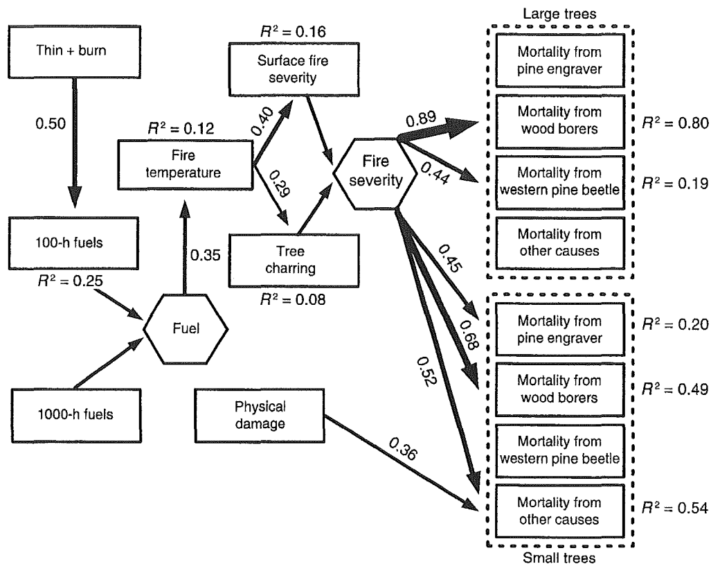
FIG. 4: Structural equation model results for large and small ponderosa pine mortality. Overall model \chi^2 = 7.86 with P = 0.10 , indicating no major deviations between data and model. Rectangles represent observed variables, while hexagons represent composites summarizing the effects of multiple predictors on individual responses. Only significant pathways are shown. Path coefficients presented are standardized values. Observed variables with pseudo- R^2 values are response variables for mortality.
