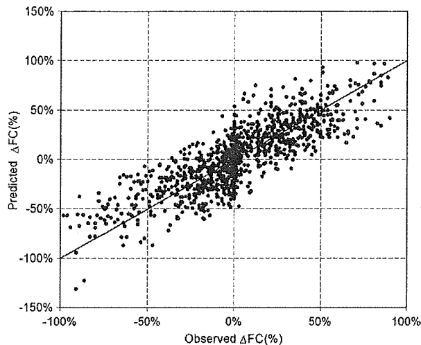
Fig. 3. Plot illustrating the relationship between the observed reference LIFC and Model 5 predicted values, based on the pooled sample set ( n = 1208 ).
