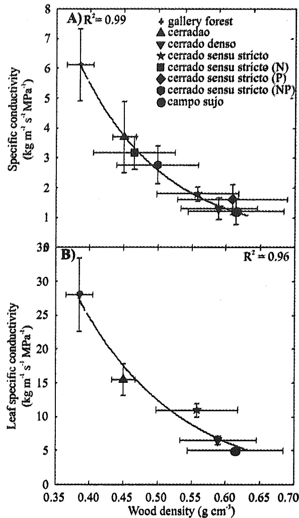
Figure 7. Specific hydraulic conductivity (a) and leaf specific hydraulic conductivity (b) in relation to weighted average wood density for sites differing in tree density (cerradao, cerrado denso, cerrado sensu stricto, campo sujo, gallery forest and cerrado sensu stricto sites subjected to long term fertilizations with N, P and N+P). Each point represents the mean value \pm SE of 10 to 16 species per site. For the gallery forest site only five dominant species were used. The lines are the exponential decaying functions fitted to the data: (a) y = 1.06 + 222 \exp(-11x) ; P < 0.05 ; (b) y = 372 \exp(-6.8x) ; P < 0.001 .
