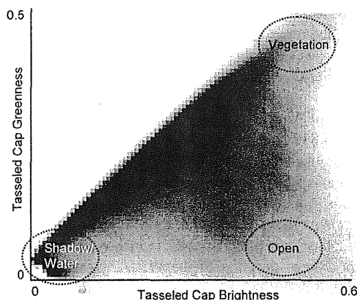
Fig. 2. Spectral end-members in Tasseled Cap brightness v. greenness space.
