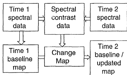
Fig. 3. An amalgam approach to change detection, where differencing is used to identify only pixels that have changed, and single date mapping rules are applied only to those changed pixels.
