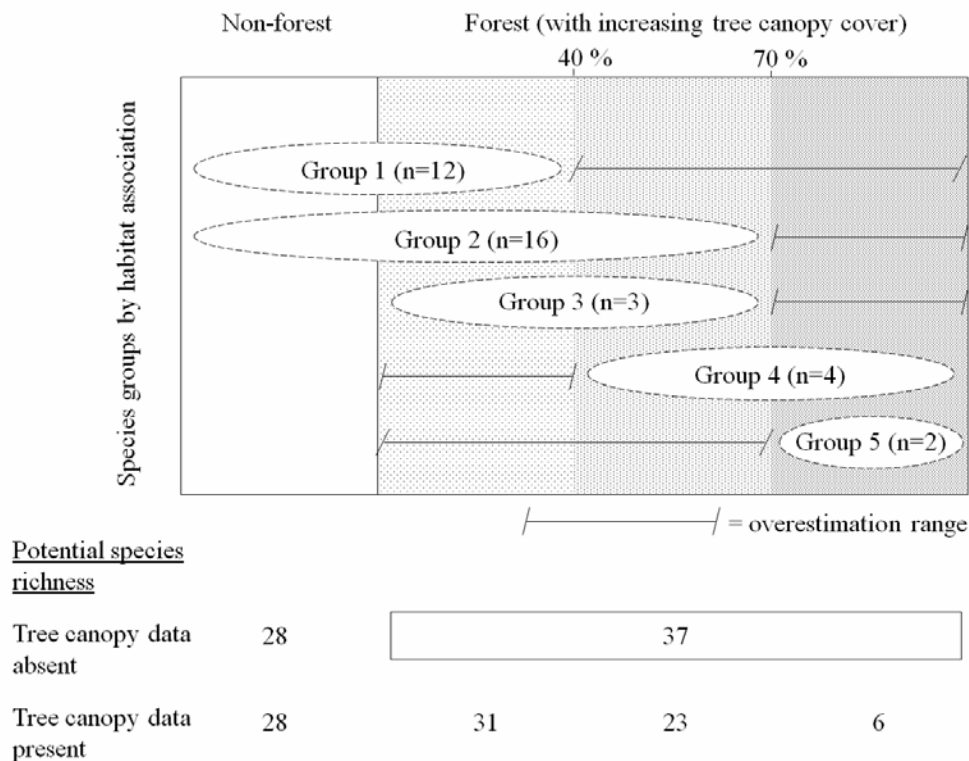
Fig. 2. Distribution of the 37 avian species according to land cover (simplified to forest/non-forest) and tree canopy cover preferences (three classes). Five groups of species were identified based on similar species-habitat relationships. Potential values of maximum species richness for scenarios with and without tree canopy information are also shown. Overestimation range refers to areas (in terms of habitat associations) where the distributions of the species have been overestimated according to the knowledge of the species' natural history.
