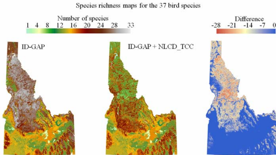
Fig. 3. Pixel based, species richness maps for the 37 avian species, including from the original ID-GAP predicted habitats and from the new ones incorporating the NLCD_TCC. The comparison of species richness between these products is also presented.
