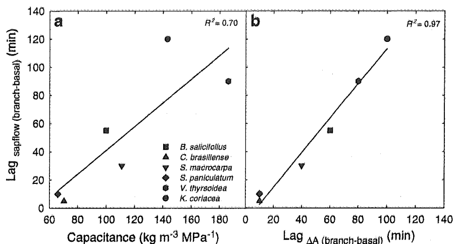
Fig. 3 The time series lag (i.e., lag corresponding to maximum correlation between time series) between branch and basal sap flow ( \text{Lag}_{\text{sapflow (branch-basal)}} ) in relation to a total stem capacitance (sapwood and outer parenchyma) and b the time series lag between branch and trunk cross-sectional area ( \text{Lag}_{\Delta A \text{ (branch-basal)}} ) for six dominant woody species of ~ Neotropical savannas. Branch and bole sap flow were measured with thermal dissipation probes and branch and bole cross sectional areas ( \Delta A ) were calculated from diameter measurements using electronic dendrometers (data from Scholz et al.,
