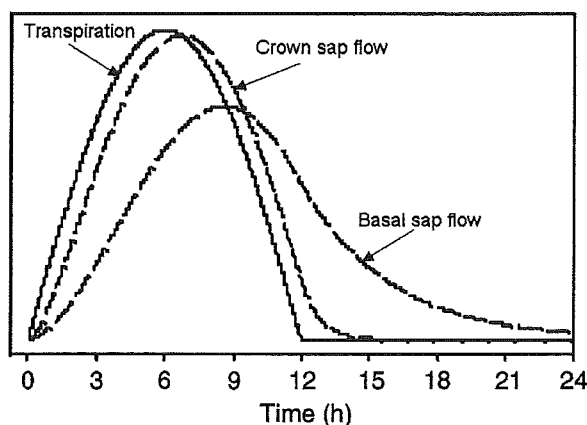
Fig. 1 Idealized time courses of transpiration (solid curve), crown sap flow (dashed curve slightly to the right of transpiration), and basal sap flow (dashed curve farther to the right). The time axis represents time of commencement of transpiration and sap fluxes, not time of day. Assumptions and interpretations of these curves are discussed in the text and Phillips et al. (2004)
