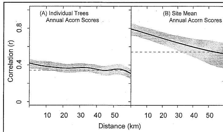
Figure 3. Spatial autocorrelation correlogram of annual acorn production from upland Puget-Willamette Trough trees (A) and local populations (B) over 8 years by distance in km with 95% confidence envelopes.
