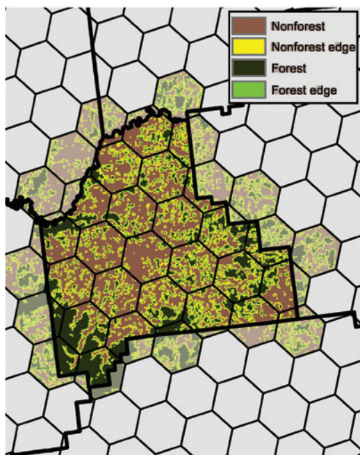
Fig. 5. Hexagon summary unit with proportional estimation method for Scott County, Indiana, USA. All pixels are counted for hexagons completely in the county (interior hexagons). For hexagons only partially in the county (boundary hexagons), all pixels are counted, and counts are multiplied by the proportion of the hexagon in the county.
