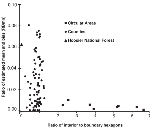
Fig. 8. Absolute value of ratio of estimated bias and pixel method stratified estimate of the mean versus ratio of interior hexagons to boundary hexagons for volume per unit area.
