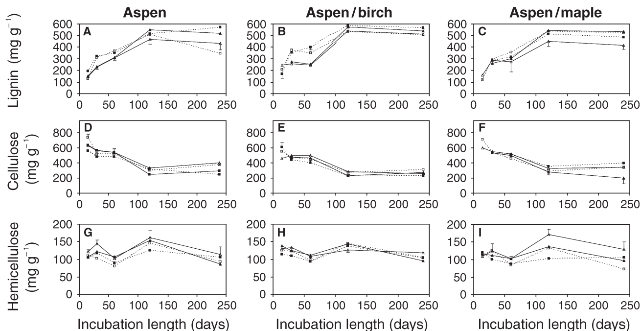
Figure 3. Mean concentrations of lignin, cellulose and hemicellulose in decomposing fine root litter (0.5–1.0 mm) produced in ambient air (control; \square ), elevated [CO 2 ] ( \blacksquare ), elevated [O 3 ] ( \triangle ), or elevated [CO 2 ] + [O 3 ] ( \blacktriangle ) at the Aspen FACE project. Bars represent standard errors of the mean (shown on one treatment only for clarity); n = 3 .
