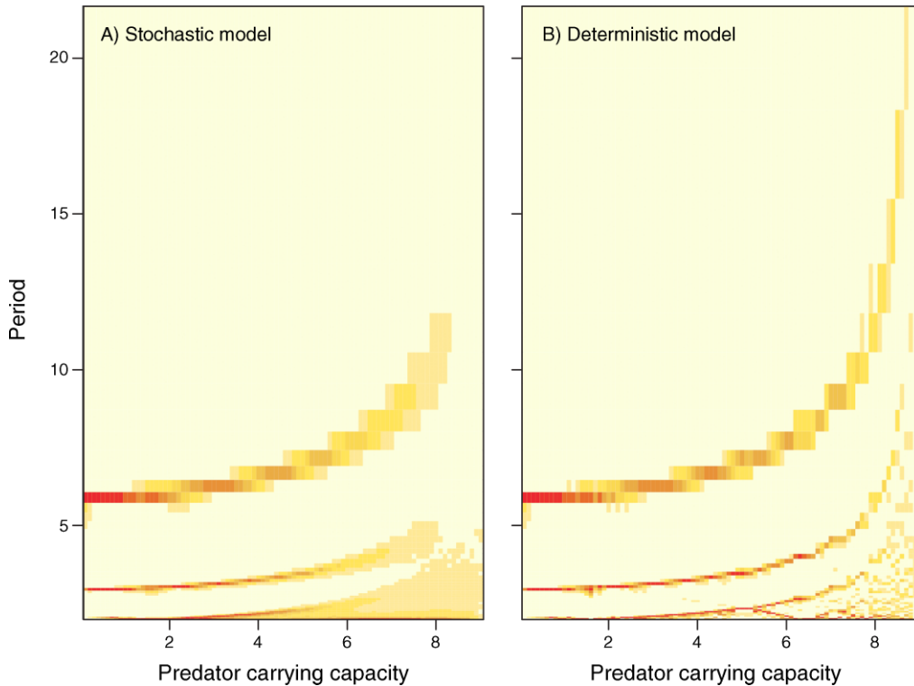
FIG. 4. Effects of predator carrying capacity on the standardized power spectra of the gypsy moth model. (A) Stochastic model and average of 500 simulations ( r = 2 , \bar{\sigma} = 0.3 ). (B) Deterministic model assuming constant predator abundance. We iterated the model for 200 generations and quantified the periodicity based on the last 100 generations.
