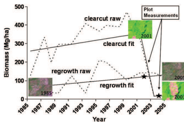
Fig. 1. Example biomass trajectories demonstrating the effect of curve-fitting (solid lines) on raw biomass predictions (dashed lines) for two recently disturbed plots. Landsat image chips centered on the plots are shown along with corresponding plot-level biomass observations.
