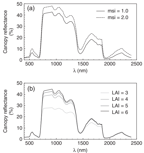
Fig. 7 Canopy reflectance values calculated via the PROSPECT-SAIL model (WinSail). (a) Increasing leaf scattering in the PROSPECT leaf model (changing mesophyll surface index, msi) increases canopy reflectance calculated via SAIL. (b) Increasing leaf area index (LAI) has a decreasing effect on reflectance and is only significant in the near infrared.
