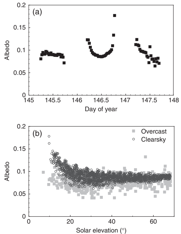
Fig. 1 (a) Variation in shortwave albedo of spruce-hemlock forest over several days. (b) Albedo as a function of solar elevation for clear sky (open circles, <40% diffuse) and overcast conditions (gray squares, >95% diffuse).
