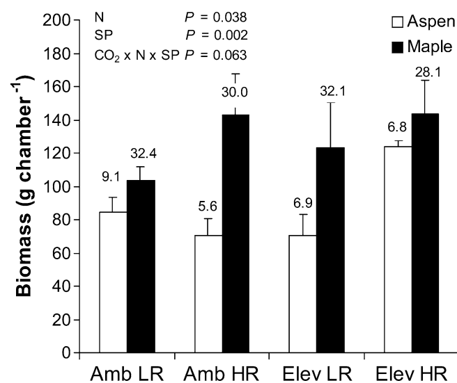
Fig. 1 Fine root biomass (<0.5 mm diameter) of trembling aspen and sugar maple produced after 2.5 growing seasons under varying atmospheric \text{CO}_2 and soil resource availability at the University of Michigan Biological Station. Values are means of dry weight scaled to the volume of soil in each chamber section ( N=4 ) and error bars are one standard error. Values over bars are the fraction (%) of total root biomass allocated to fine roots. “Amb”, “Elev” denote ambient and elevated \text{CO}_2 treatments, respectively; “LR”, “HR” denote the low and high soil resource availability treatments, respectively
