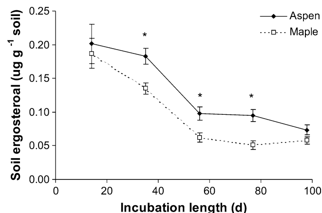
Fig. 3 Soil ergosterol content in the experimental soil mix from the 98-day laboratory incubation of trembling aspen and sugar maple fine roots produced after 2.5 growing seasons under varying atmospheric CO 2 and soil resource availability at the University of Michigan Biological Station. Values are averaged over the non-significant factors of atmospheric CO 2 and soil resource availability ( N=16 ) and error bars are one standard error (shown on one treatment only for clarity). *Denotes significant at P \leq 0.05 . Data adapted from Schmidt (2000)
