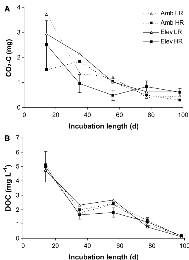
Fig. 2 Microbially respired CO 2 -C (a) and dissolved organic carbon (b) from the 98-day incubation of fine roots from trembling aspen and sugar maple produced after 2.5 growing seasons under varying atmospheric CO 2 and soil resource availability at the University of Michigan Biological Station. Values were averaged over the non-significant factor species ( N=8 ), and error bars are one standard error (shown on one treatment only for clarity). Treatment legend is the same as Fig. 1. Data adapted from Schmidt (2000)
