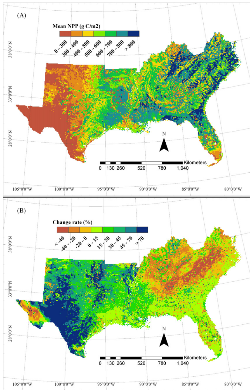
Fig. 7. Spatial distribution of annual mean NPP across the terrestrial ecosystems of the southern United States during 1895–2007 (g C/m 2 /yr, A) and NPP change rate (% B) from 1961–1990 to 1991–2007.
