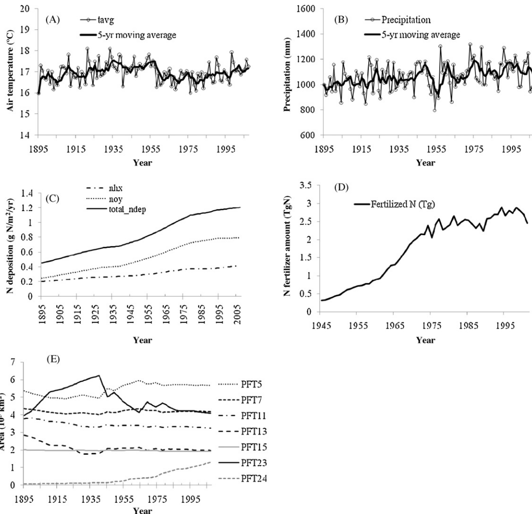
Fig. 3. Magnitude of changes in multiple environmental factors in the southern United States. Note: nhx, deposited nitrogen as the form of \text{NH}_x\text{-N} including \text{NH}_3 and \text{NH}_4^{+}\text{-N} ; noy, deposited nitrogen as the form of \text{NO}_y\text{-N} including all oxidized forms of nitrogen except \text{N}_2\text{O} . (A) Mean annual temperature ( ^{\circ}\text{C} ) from 1895 to 2007; (B) annual precipitation (mm) from 1895 to 2007; (C) N deposition rate ( \text{g N/m}^2/\text{yr} ) from 1895 to 2007; (D) N fertilizer amounts (Tg N) in the cropland from 1945 to 2001; (E) area of different biomes from 1895 to 2007 (PFT5: temperate deciduous broadleaf forest; PFT7: temperate evergreen needleleaf forest (including mixed forest); PFT11: deciduous shrubland; PFT13: C 3 and C 4 grassland; PFT15: grass and forest wetland; PFT23: cropland; PFT24: build-up land).
