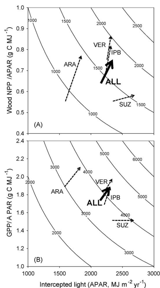
Fig. 5. The irrigation effect on (A) wood growth and (B) gross primary productivity (GPP) depended on changes in light capture (APAR) and efficiency of light use. These graphs show production as contour lines; horizontal vectors show the magnitude of the effect of increased APAR, and vertical vectors show the effect of increased light-use efficiency. The beginning of each arrow indicates the values for the unirrigated treatment, and the end of the arrow indicates the value for the irrigated treatment. The average vector across all sites angled at more than 45^\circ from horizontal, indicating that gains in efficiency were more important than gains in APAR.
