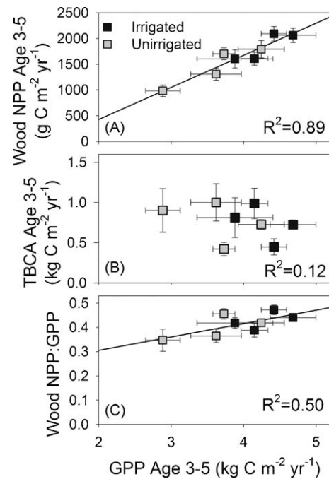
Fig. 2. Wood net primary productivity (NPP) increases with (A) annual photosynthesis (GPP) via two mechanisms: higher carbohydrate supply (GPP) and (C) increased partitioning to wood NPP. Flux to TBCF (B) does not vary with GPP for these sites and treatments. Error bars are standard errors for treatment means for each of the four sites, computed from the age three to five plot means.
