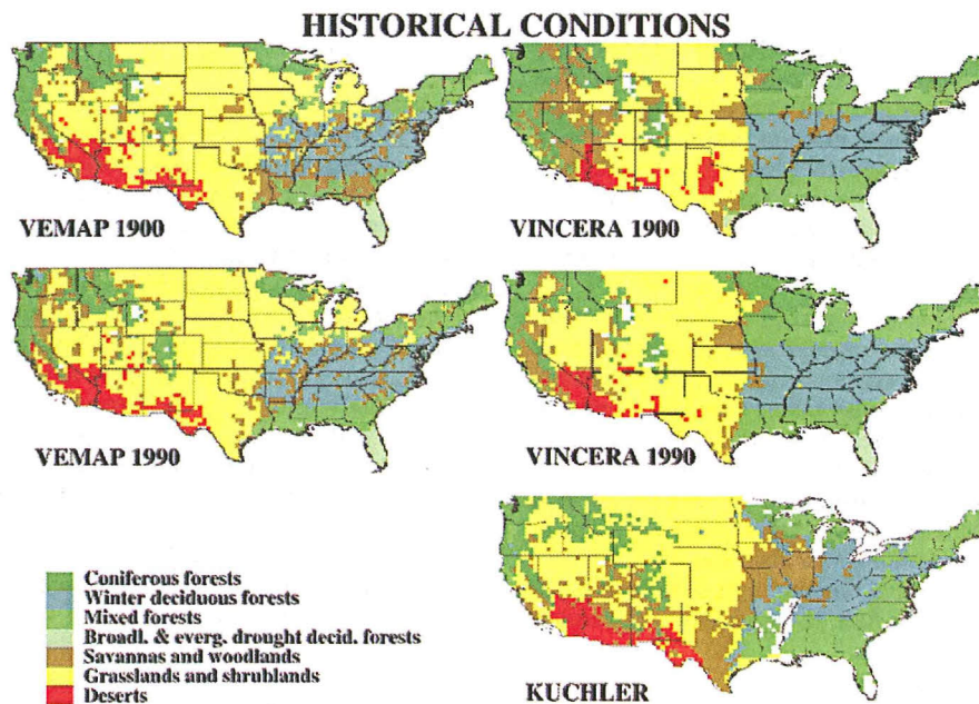
Fig. 3. Distribution of aggregated vegetation classes (modal average) simulated by MC1 under VEMAP and VINCERA historical climate compared with a map derived from Küchler (1964). The model assumes a continuous increase in the atmospheric CO 2 concentration from 295 ppm in 1895 to 354 ppm in 1990.
