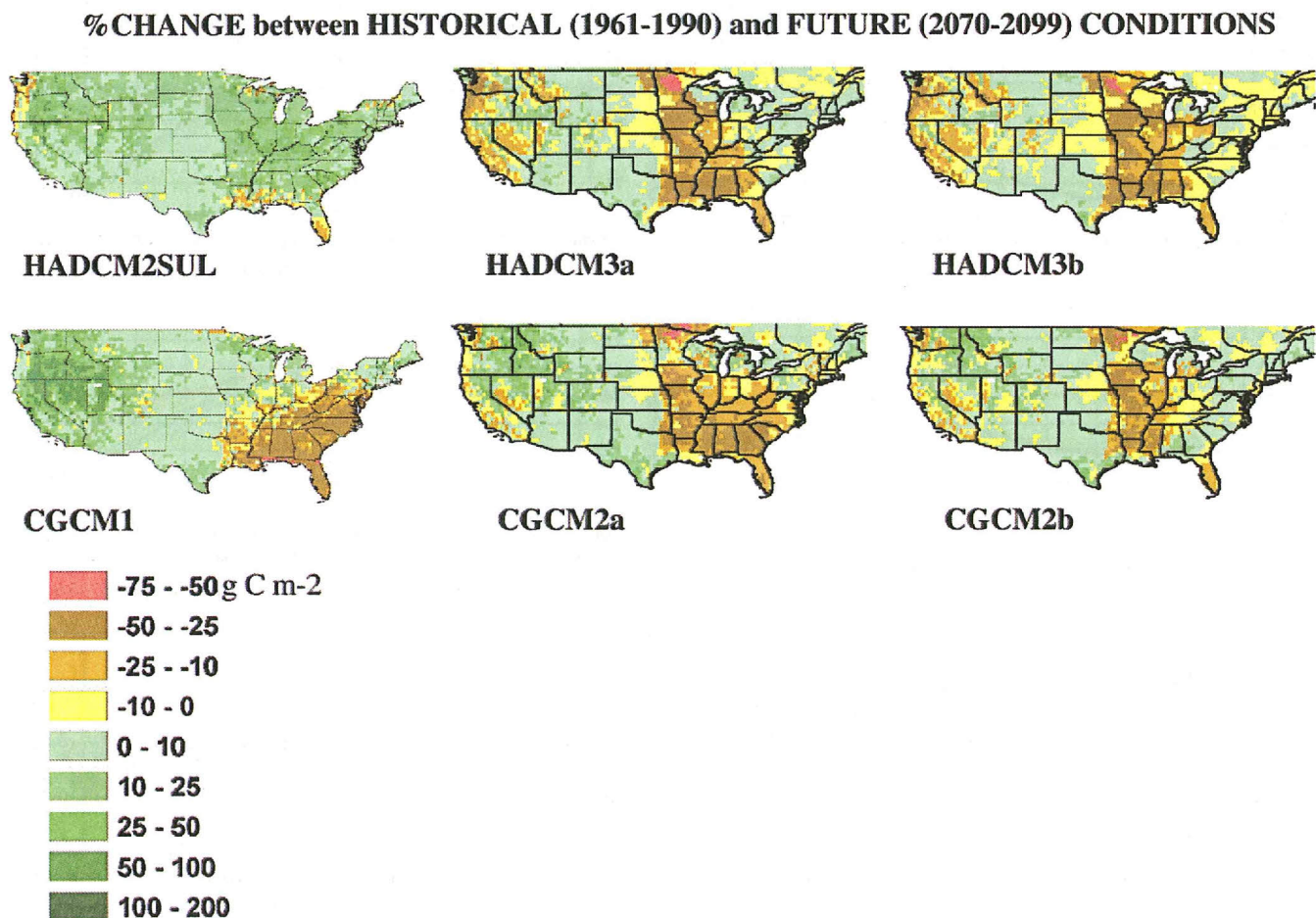
Fig. 5. Change in total carbon storage simulated by MC1 under VEMAP and VINCERA from 1895 to 2100. The model assumes a continuous increase in the atmospheric CO 2 concentration from 295 ppm in 1895 to 712 ppm in 2100 under VEMAP, 605 ppm under SRES A and 823 ppm under SRES B in 2100 for VINCERA.
