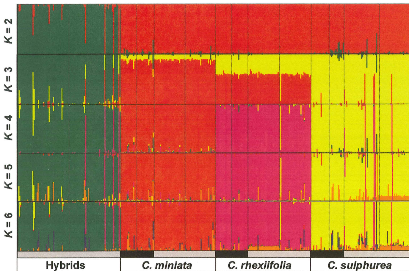
Fig. 8. Population structure and individual admixture for Castilleja as revealed by AFLP banding patterns under different assumptions of K (the number of clusters) from 2 to 6. Each individual is represented by a line that is partitioned into sections that depict the individual's estimated membership into each of the K clusters. Samples from "pure parental" populations are indicated by a black bar above the species name; samples from "comingled" and "hybrid" populations are indicated by a gray bar.
