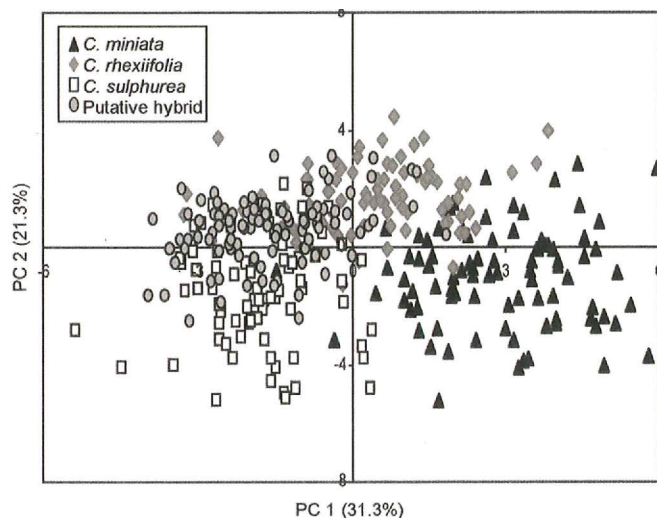
Fig. 3. Principal component analysis of 17 quantitative traits for the three Castilleja species and their putative hybrids showing the principal component (PC) scores for PC1 vs. PC2. The percentage variation explained by each axis is given in parentheses.
