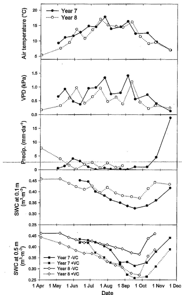
Figure 1. Mean air temperature, daytime vapor pressure deficit (VPD), daily precipitation, and mean soil water content (SWC) at 0.1- and 0.5-m depths during each dendrometer measurement period. Because SWC differed by vegetation control (VC) treatment at 0.5 m, both treatments are shown.
