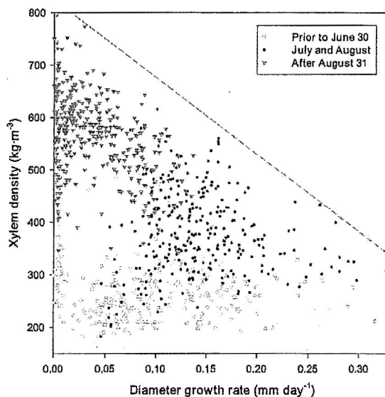
Figure 4. Relationship between diameter growth rate and xylem density for Douglas-fir during two growing seasons; each point represents an approximate 2-wk measurement period for one tree. Data trended in a counterclockwise pattern throughout the growing season; for clarity, the growing season has been divided into three periods.
