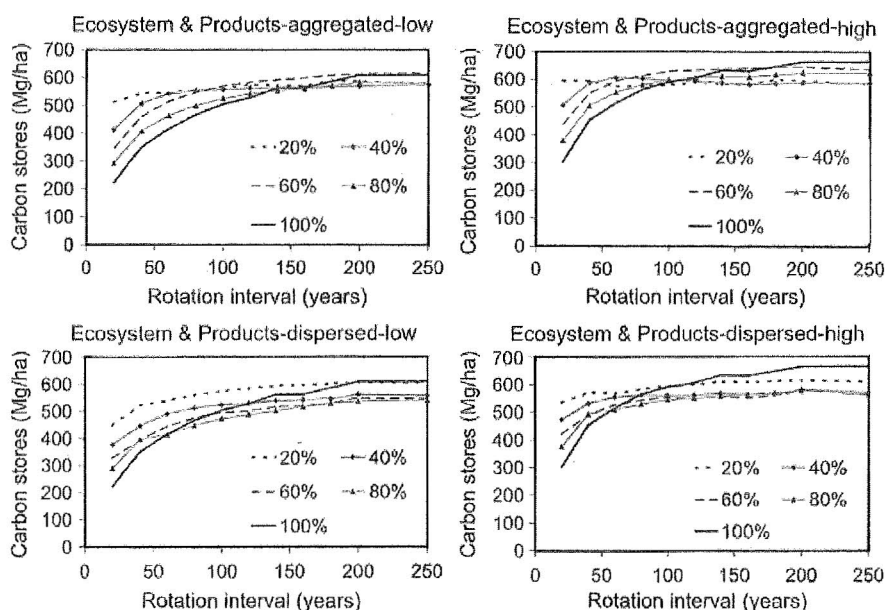
Figure 9. Average total system (ecosystem and forest products) C stores over a harvest rotation interval for different levels of removal (percent of cells harvested) and cutting patterns. Aggregated represents one contiguous harvest block and dispersed represents a checkerboard pattern of harvest-no harvest. Low represents a system in which 50% of the harvested C is converted to long-term forest products with losses of 2% per year; high represents a system in which 75% is converted to long-term forest products with losses of 1% per year.
