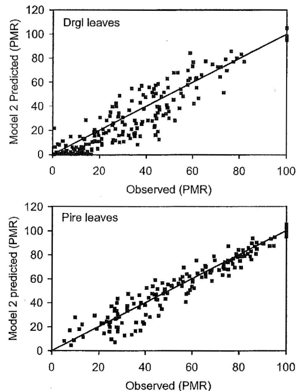
Fig. 6 Remaining mass predicted by the simple negative exponential regression with initial mass constrained to 100% (Model 2) vs. the observed data for two representative litter types. PMR is percent mass remaining; the 1:1 line is shown.
