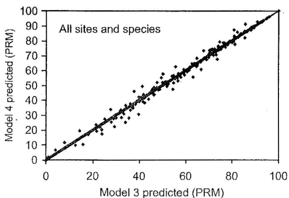
Fig. 8 Relationship between predictions of Models 3 and 4. Both models are negative exponential and asymptotic regressions, but Model 4 has the initial mass constrained to 100%. PMR is percent mass remaining; the 1:1 line is shown.
