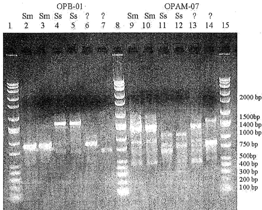
Fig. 3. Banding patterns for Scolytus multistriatus (Sm; lanes 2, 3, 9, and 10), S. schevyrewi (Ss; lanes 4, 5, 11, and 12), and four of eight individuals of Scolytus spp. not identifiable using current taxonomic criteria (?; lanes 6, 7, 13, and 14) with each primer. Lanes 2–7 show banding patterns from OPB-01; lanes 9–14 show banding patterns from OPAM-07, and lanes 1, 8, and 15 indicate molecular weights.
