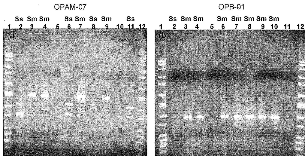
Fig. 4. (a) Blind test validating species-specific banding patterns using the oligonucleotide OPAM-07. Scolytus schevyrewi : lanes 2, 6, 8, and 11; S. multistriatus : lanes 3, 4, 7, and 9. (b) Results for larvae with primer OPB-01. Lane 2: S. schevyrewi ; lanes 3–10: S. multistriatus .
