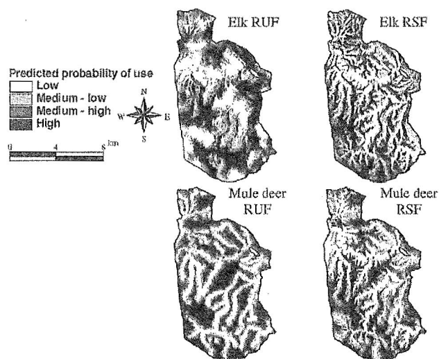
Figure 1. Predicted relative probability of use by elk ( n=75 ) and mule deer ( n=39 ) in Main Study Area, Starkey Experimental Forest and Range, Oregon, USA, generated from resource utilization functions (RUFs) and resource selection functions (RSFs). We based models of resource selection on location data collected with a LORAN-C automated telemetry system during spring (30 Apr–14 Jun) of 1999–2001 within 1 hour of sunrise or sunset.
