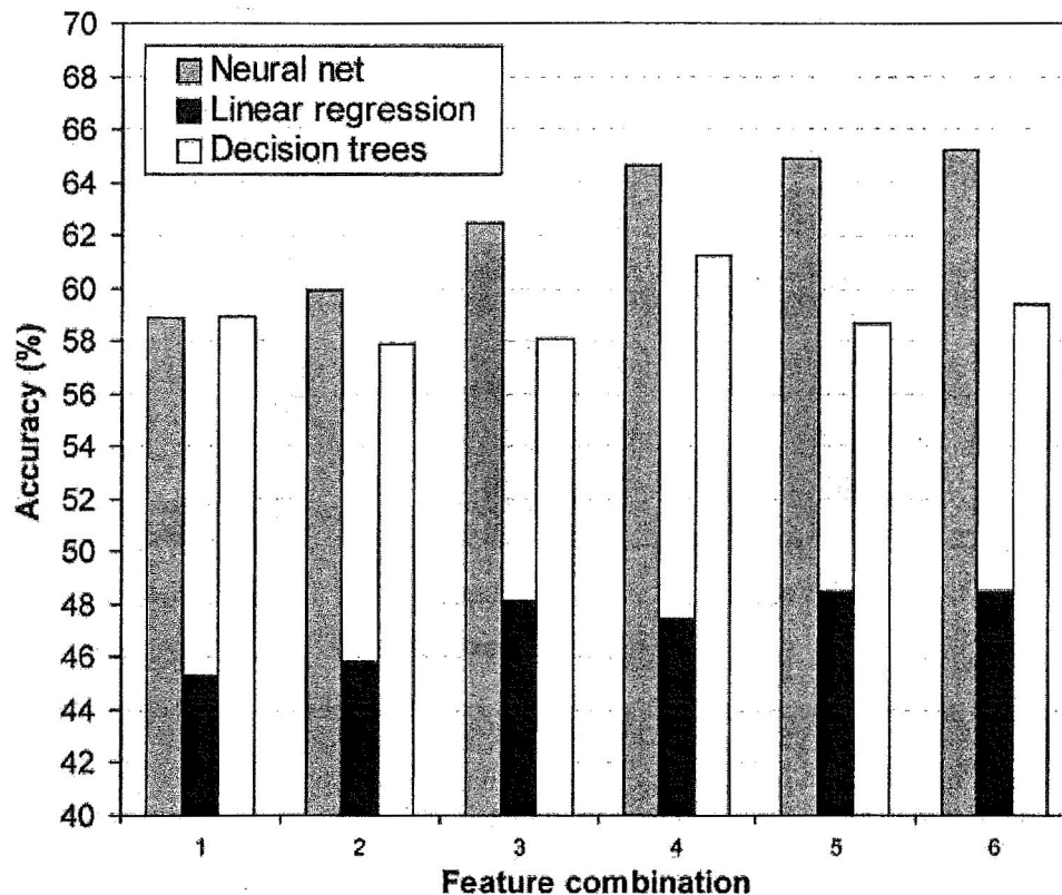
Figure 4. Predictive accuracy of models with six feature combinations in table 2 and three successional stages: young (age < 50 years), mature (age 51–149 years) and old (age > 150 years).
