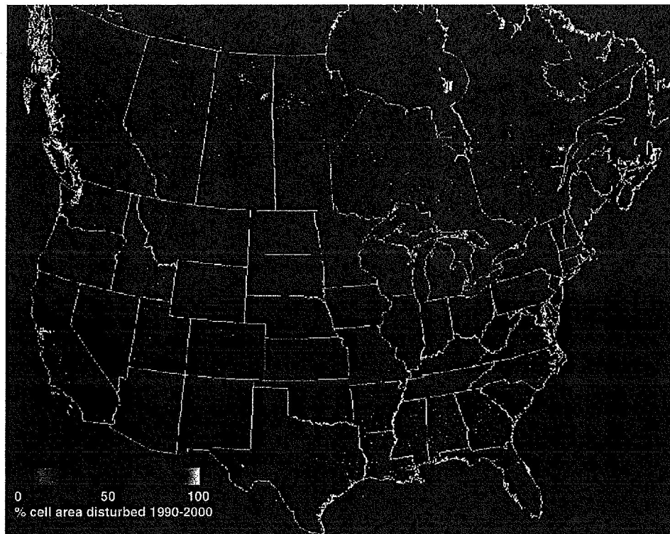
Fig. 11. Stand-clearing disturbance rates for conterminous United States and Canada, 1990–2000. Values are expressed in percent of 500×500 m cell area disturbed during the nominal 1990–2000 period.
