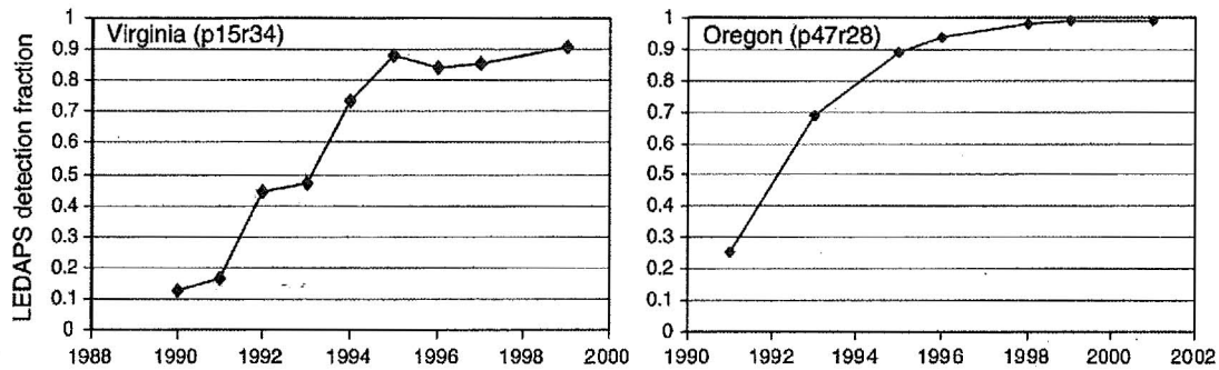
Fig. 6. Example of LEDAPS detection accuracy (1-omission error) as function of actual disturbance date for two 15×15 km subsets in Virginia (left) and Oregon (right). Disturbance date was determined with a precision of <2 years for reference data sets using the approaches described in the text. Detection accuracy of LEDAPS products drops for older disturbances, since regeneration masks the spectral signal by the end of the 10-year observation interval.
