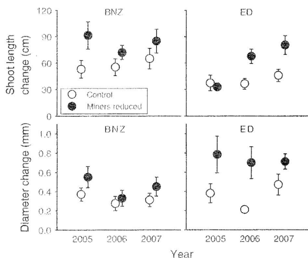
Fig. 2 Two measures of growth by trees that were sprayed to reduce leaf miner damage (black circles) and unsprayed controls (white circles) at two study sites during the 2005, 2006, and 2007 growing seasons. Error bars are SEM. BNZ Bonanza Creek Long-Term Ecological Research Site, ED Ester Dome site
