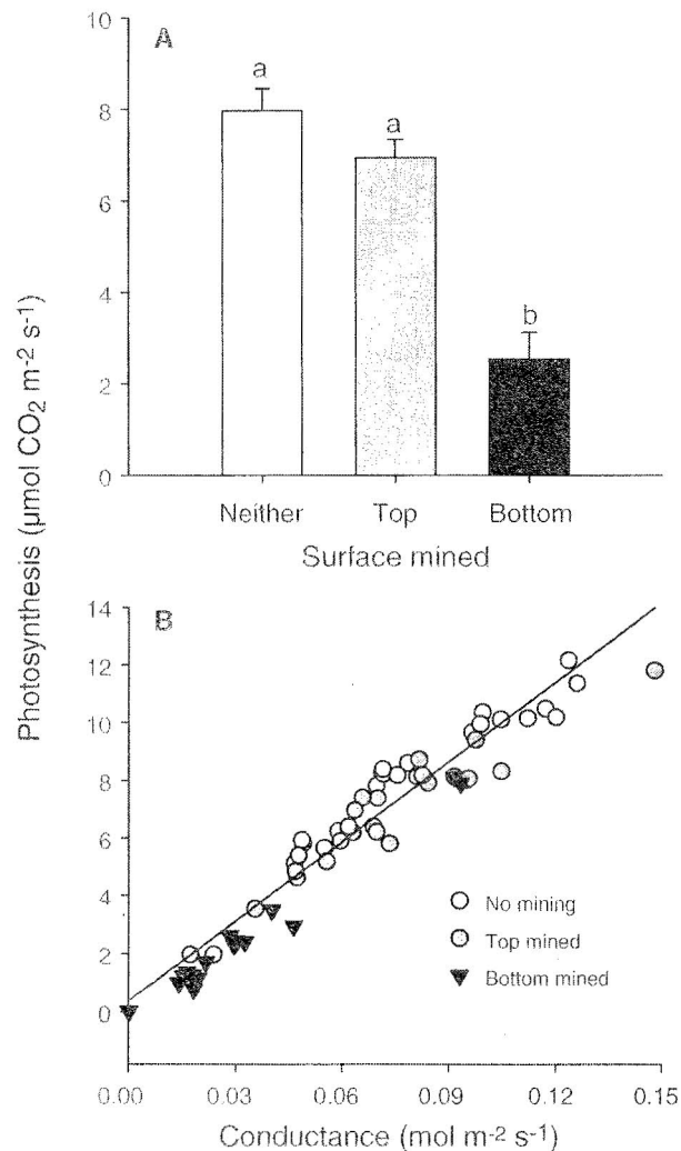
Fig. 4 Gas exchange by leaves on which the presence and location of leaf miners was experimentally manipulated. a Photosynthesis by leaves with no mining damage ( Neither ; n = 26 ), damage to the leaf top only ( Top ; n = 23 ), and damage to the leaf bottom only ( Bottom ; n = 17 ). Bars annotated with different lowercase letters were significantly different using Tukey–Kramer honestly significant difference test ( P < 0.05 ). b The relationship between photosynthesis and water vapor conductance for the same leaves
