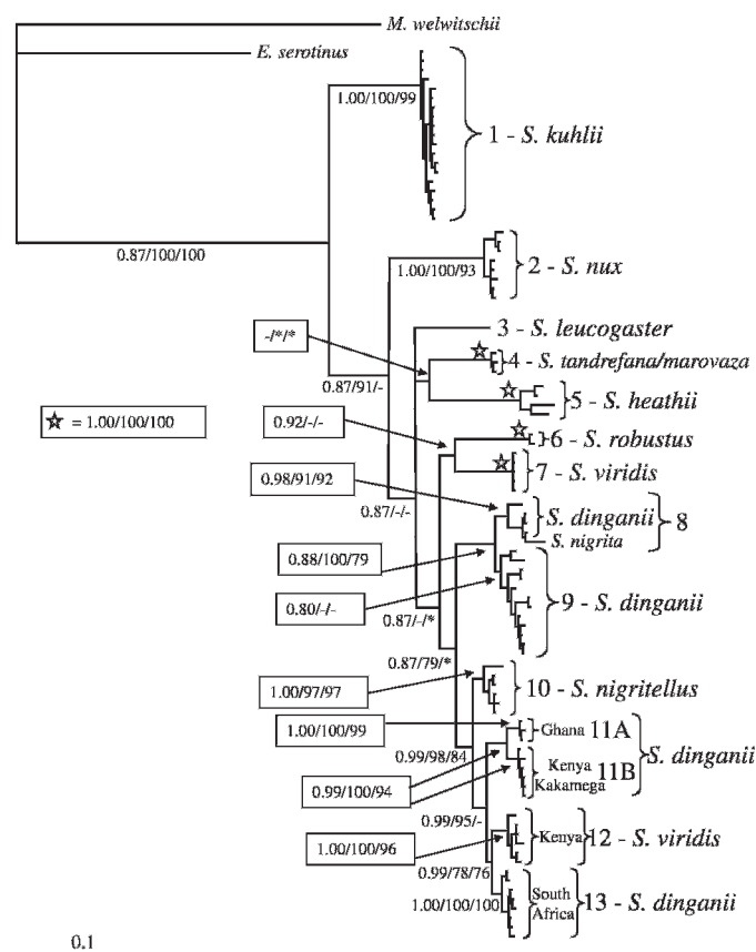
FIG. 1. —Bayesian phylogram from analysis of cytochrome- b gene sequences (1,140 base pairs). Myotis welwitschii and Eptesicus serotinus were designated as outgroup taxa. Numbers in boxes represent node support (Bayesian posterior probabilities/parsimony bootstrap percentages/maximum-likelihood bootstrap percentages). All nodes shown are supported by posterior probability or bootstrap values > 50 or 0.50 in at least 1 of the analyses. Support values are only shown for those nodes supported by posterior probability or bootstrap percent \geq 70 ( 0.70 Bayesian posterior probability). Values designated with (-) are support values > 50 but < 70 ( 0.50 and 0.70 for Bayesian posterior probability) and those designated (*) are nodes with support values < 50 and indicate collapsed nodes in that particular analysis. Clades mentioned in the text are numbered 1–13.
