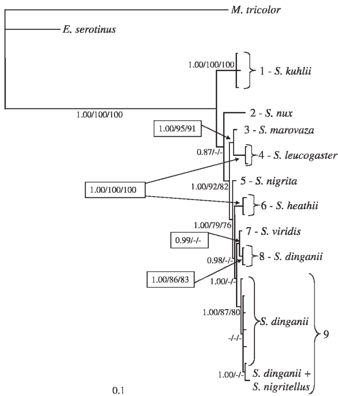
FIG. 2.—Bayesian phylogram from analysis of partial sequences of the zfy gene (2,283 base pairs). Myotis tricolor and Eptesicus serotinus were designated as outgroups. Node support is designated as in Fig. 1. Clades mentioned in the text are numbered 1–9.
