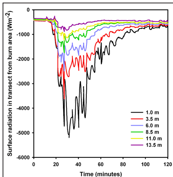
Figure 2. Time course of one-minute-mean surface radiant energy flux measured outside the burn area during an April 2004 experimental slash-pile burn performed at the Manitou Experimental Forest, located in the Rocky Mountains of Central Colorado (Massman et al. 2007), using water-cooled Medtherm Corp. (Huntsville, Alabama, USA) Series 64 heat flux transducers spaced radially between 1.0 m to 13.5 m from the edge of the pile. Negative fluxes indicate that the heat flow is downward or into the soil. For the purposes of documenting the temporal sequence of events depicted in this figure and the next three figures, it should be noted that the fire was initiated at the edge of the slash pile at 10:10 AM on day 117 = 117.43 of 2004.
