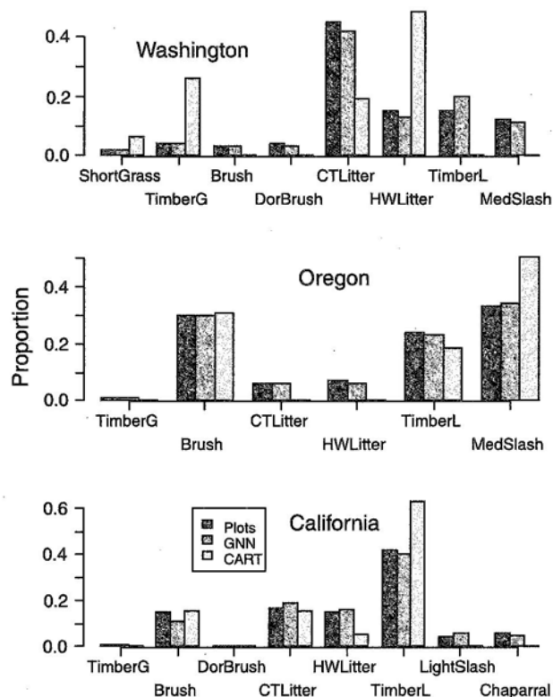
Fig. 5. Distribution of forest area among fuel models from plot-based estimates and from spatial predictions from gradient nearest neighbor (GNN) and classification and regression trees (CART). See Table 2 for definitions of fuel models.
