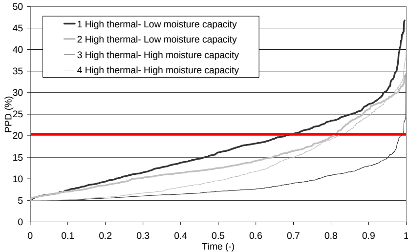
Figure 1. Duration curve of predicted percentage of dissatisfied for constructions with high thermal capacity, in August.
