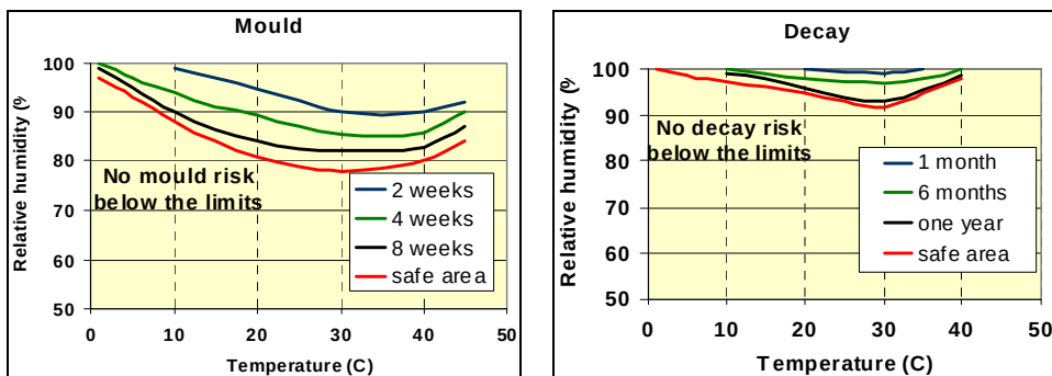
Figure 4 a and b. Humidity and temperature isopleths for mould and decay to develop in untreated pine sapwood.
