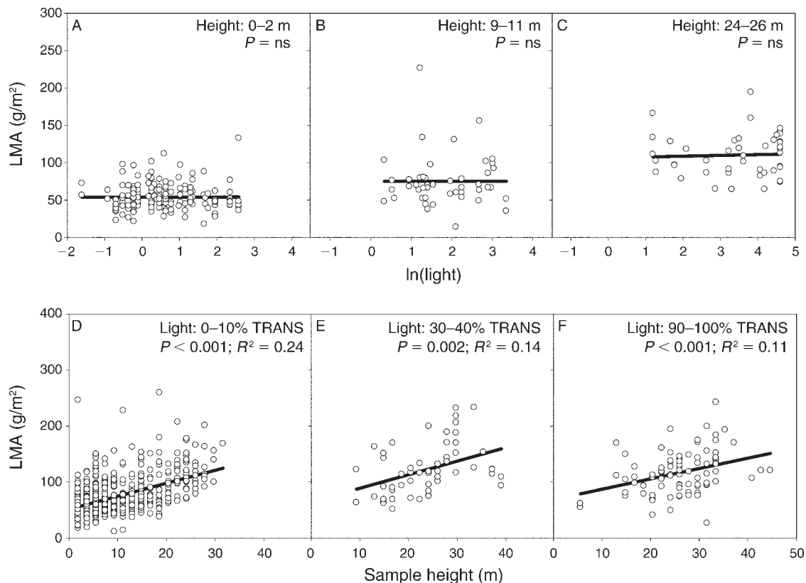
FIG. 5. For all functional groups pooled, LMA is plotted against \ln(\text{light}) for three narrow bands of height (panels A–C), and against height for three narrow bands of light (panels D–F). Figures show no change in LMA with light at three height levels, but significant increase in LMA with height at three light levels. The abbreviation “ns” indicates not significant.
