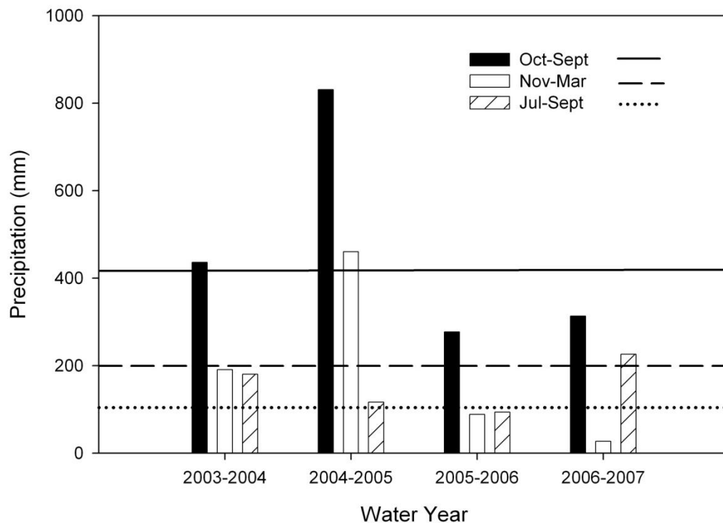
Fig. 2.1 Annual water year precipitation near the study site (Nixon Flats Remote Access Weather Station). Bars represent total water year (October to September), winter (November to March), and monsoonal (July to September) precipitation. The lines represent the 1992-2007 average precipitation. The solid line is the annual average, the dashed line is the winter average, and the dotted line is the monsoonal average
